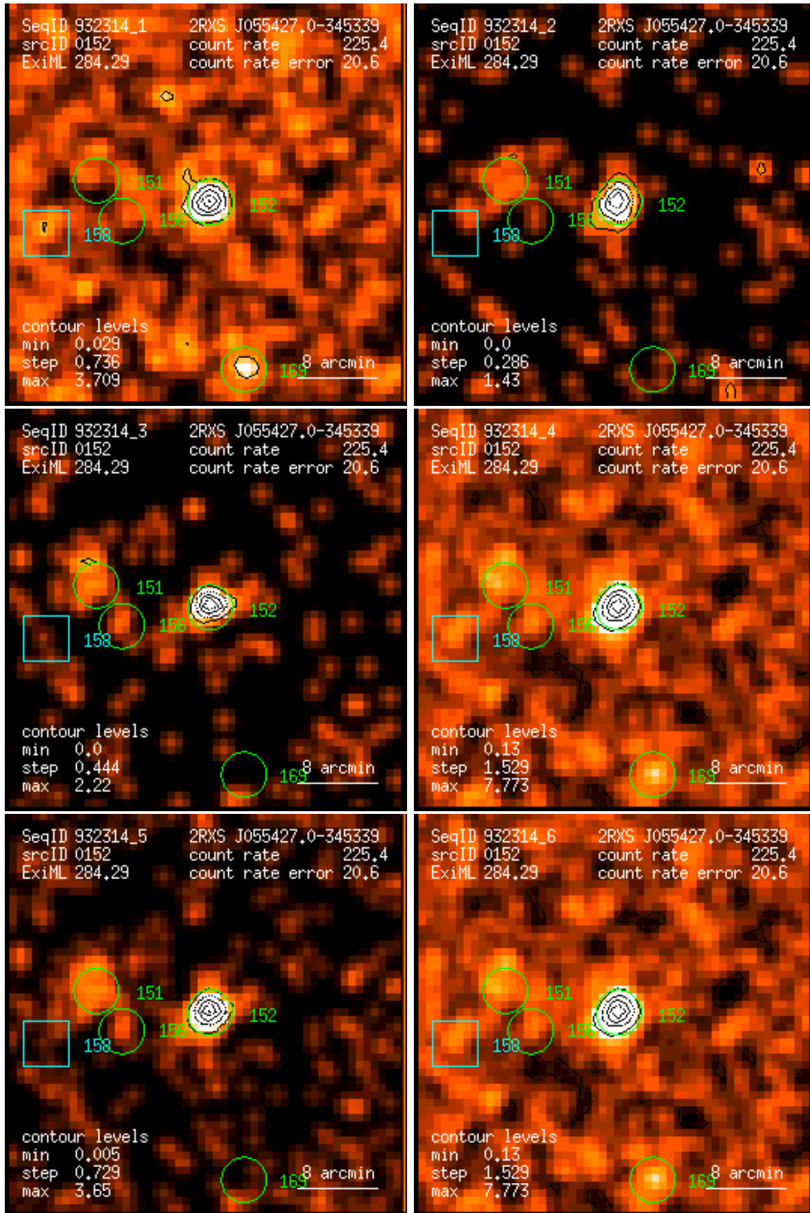
Figure 152: RASS 932314: detection 0152: band rate images, Gaussian filter: (1) PSPC channels 11 – 41, (2) 52 – 90, (3) 91 – 201, (4) 11 – 235, (5) 52 – 201, (6) 11 – 201. Broad band rates in counts/ks. Band rate contour levels in counts/ks/arcmin 2 .
