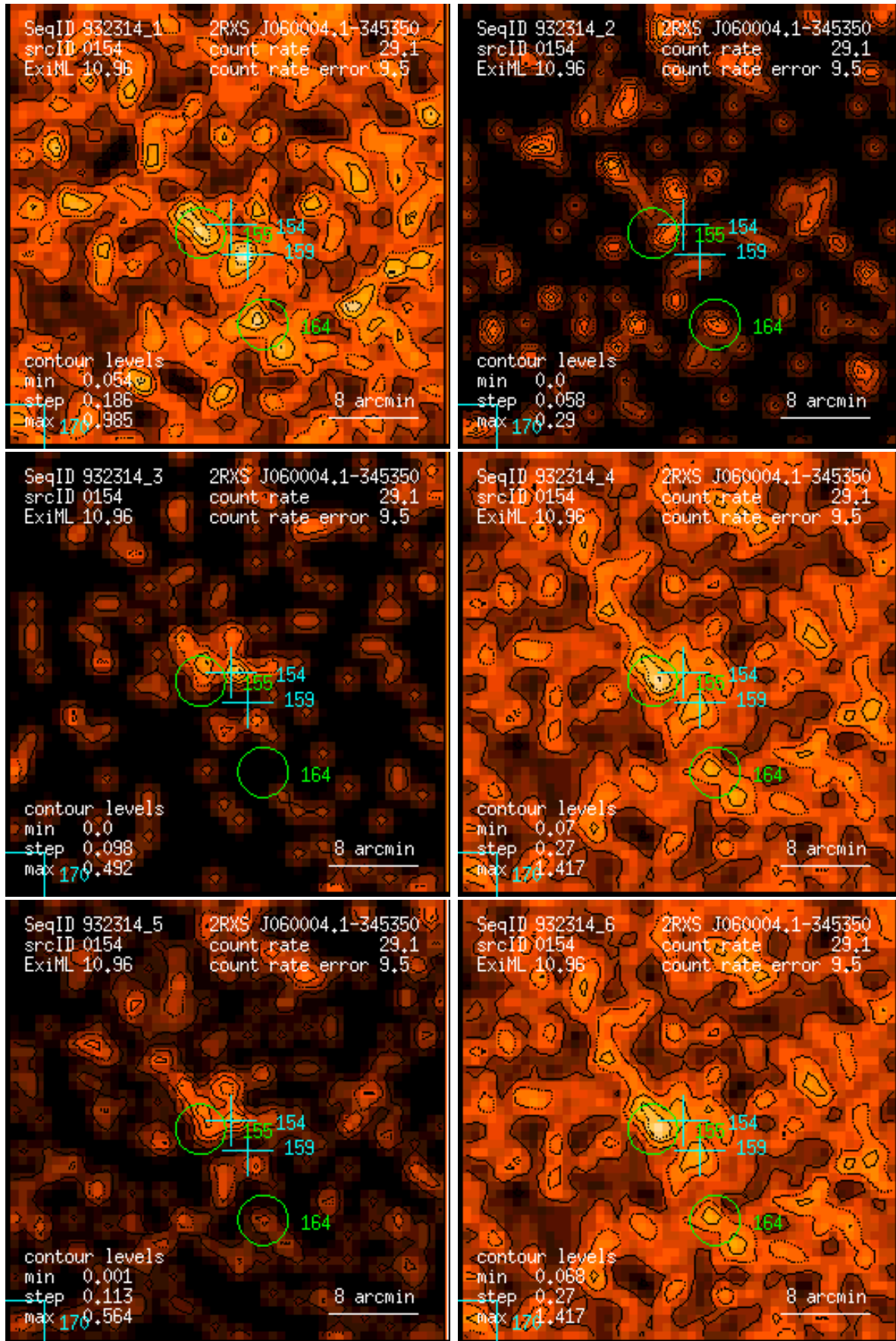
Figure 154: RASS 932314: detection 0154: band rate images, Gaussian filter: (1) PSPC channels 11 – 41, (2) 52 – 90, (3) 91 – 201, (4) 11 – 235, (5) 52 – 201, (6) 11 – 201. Broad band rates in counts/ks. Band rate contour levels in counts/ks/arcmin 2 .
