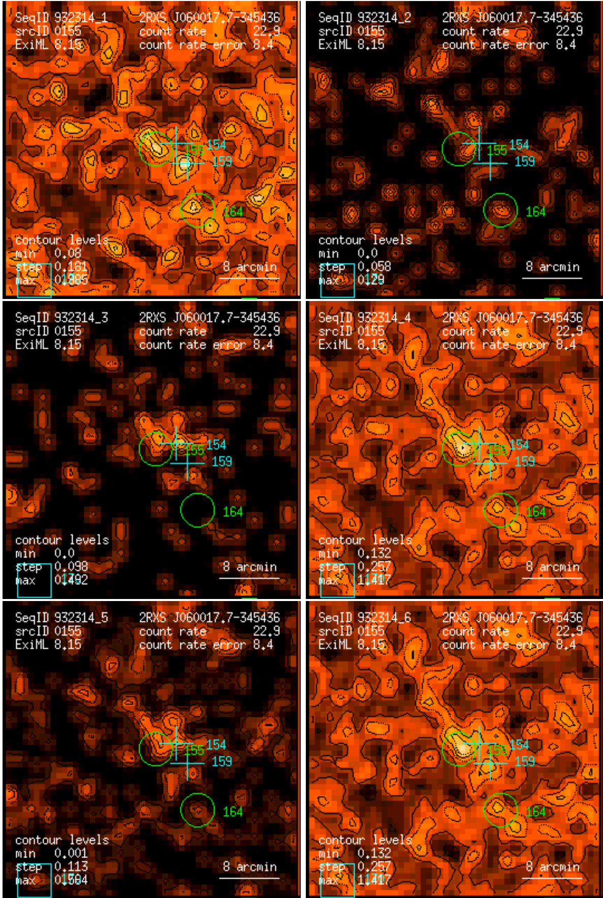
Figure 155: RASS 932314: detection 0155: band rate images, Gaussian filter: (1) PSPC channels 11 – 41, (2) 52 – 90, (3) 91 – 201, (4) 11 – 235, (5) 52 – 201, (6) 11 – 201. Broad band rates in counts/ks. Band rate contour levels in counts/ks/arcmin 2 .
