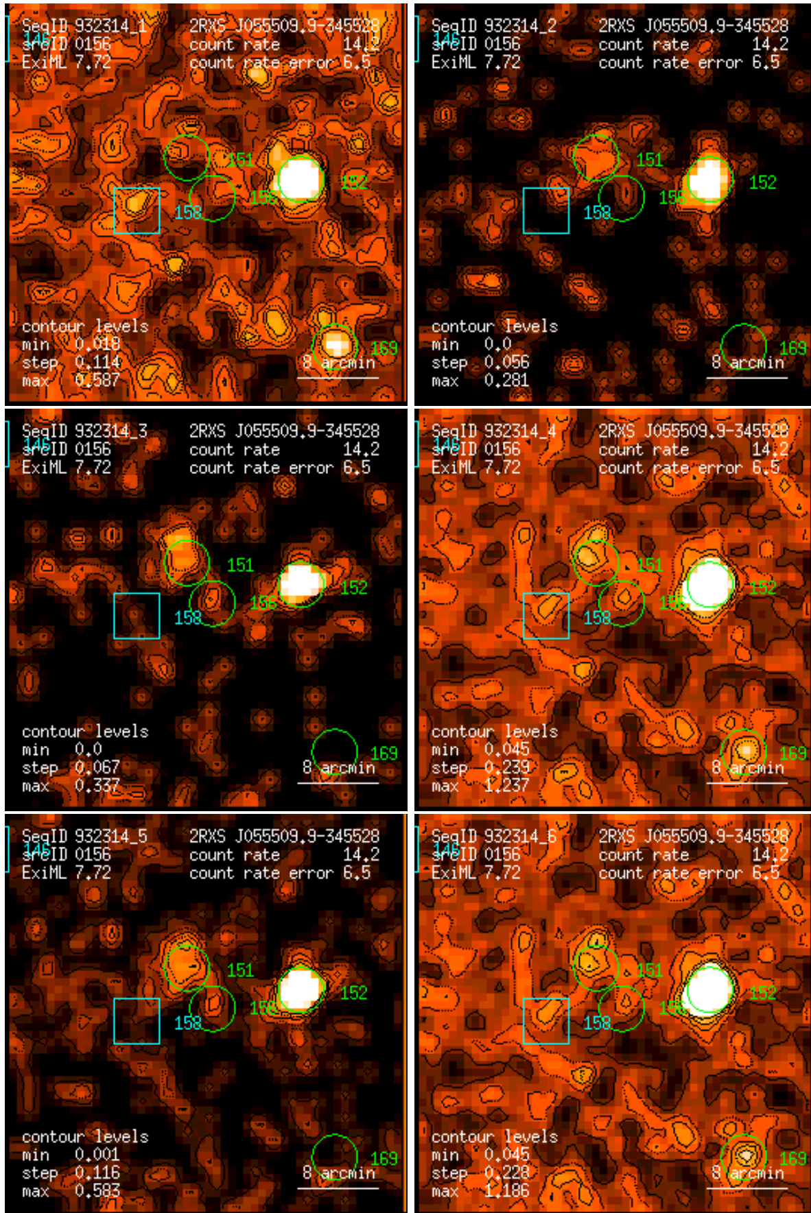
Figure 156: RASS 932314: detection 0156: band rate images, Gaussian filter: (1) PSPC channels 11 – 41, (2) 52 – 90, (3) 91 – 201, (4) 11 – 235, (5) 52 – 201, (6) 11 – 201. Broad band rates in counts/ks. Band rate contour levels in counts/ks/arcmin 2 .
