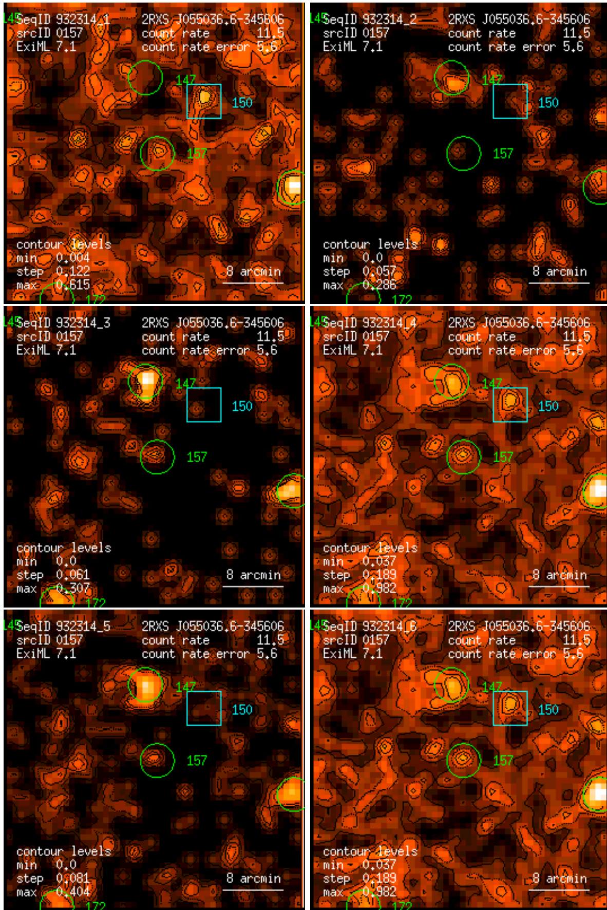
Figure 157: RASS 932314: detection 0157: band rate images, Gaussian filter: (1) PSPC channels 11 – 41, (2) 52 – 90, (3) 91 – 201, (4) 11 – 235, (5) 52 – 201, (6) 11 – 201. Broad band rates in counts/ks. Band rate contour levels in counts/ks/arcmin 2 .
