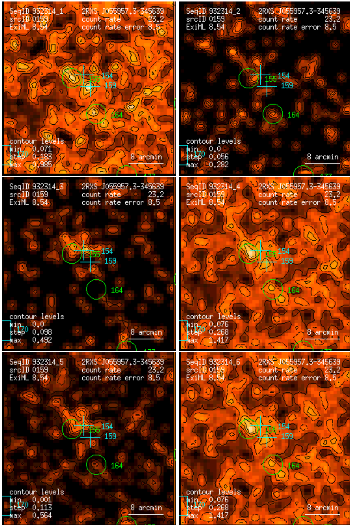
Figure 159: RASS 932314: detection 0159: band rate images, Gaussian filter: (1) PSPC channels 11 – 41, (2) 52 – 90, (3) 91 – 201, (4) 11 – 235, (5) 52 – 201, (6) 11 – 201. Broad band rates in counts/ks. Band rate contour levels in counts/ks/arcmin 2 .
