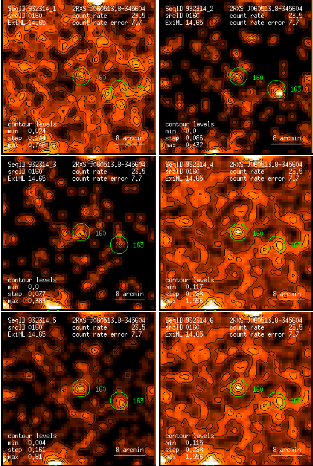
Figure 160: RASS 932314: detection 0160: band rate images, Gaussian filter: (1) PSPC channels 11 – 41, (2) 52 – 90, (3) 91 – 201, (4) 11 – 235, (5) 52 – 201, (6) 11 – 201. Broad band rates in counts/ks. Band rate contour levels in counts/ks/arcmin 2 .
