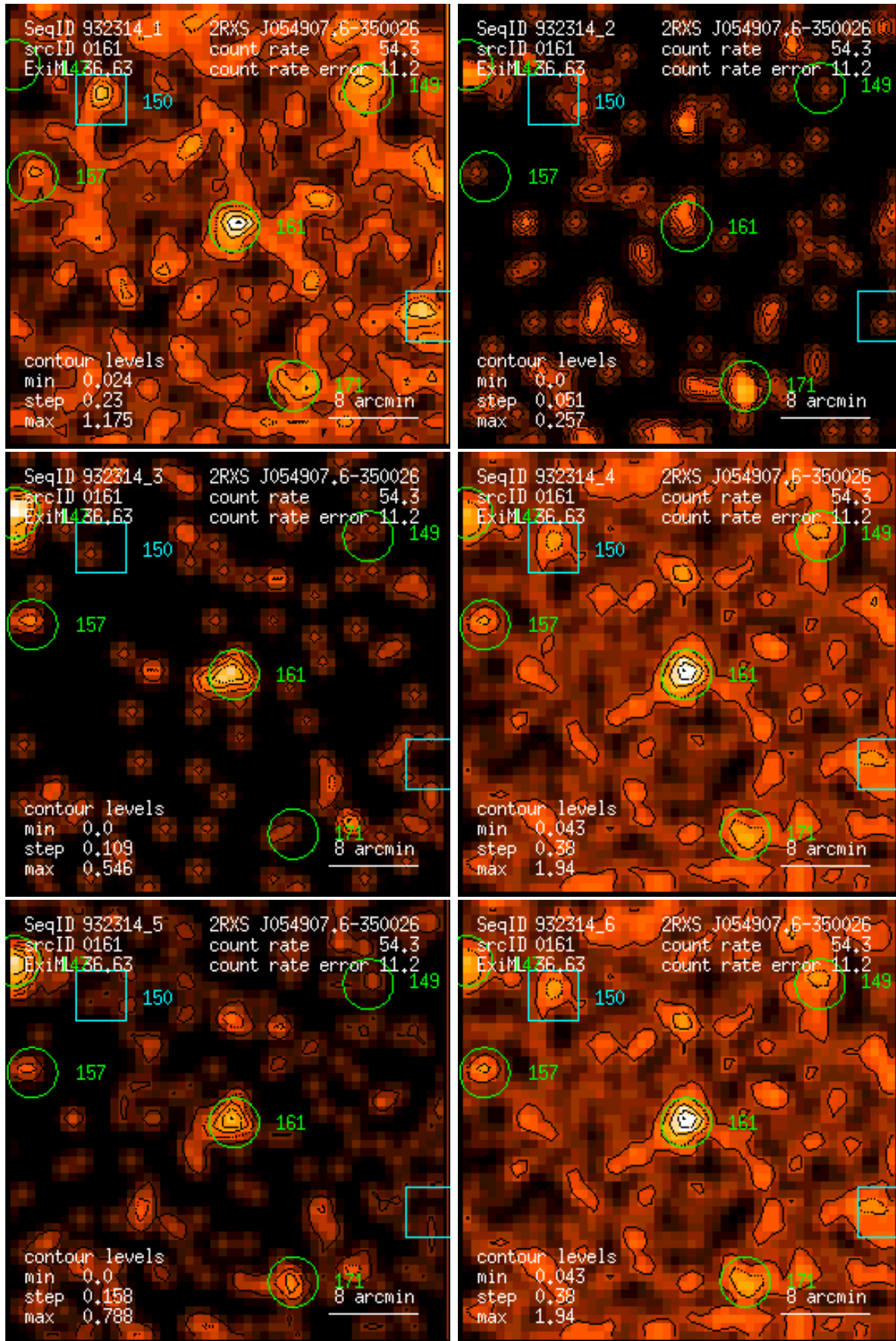
Figure 161: RASS 932314: detection 0161: band rate images, Gaussian filter: (1) PSPC channels 11 – 41, (2) 52 – 90, (3) 91 – 201, (4) 11 – 235, (5) 52 – 201, (6) 11 – 201. Broad band rates in counts/ks. Band rate contour levels in counts/ks/arcmin 2 .
