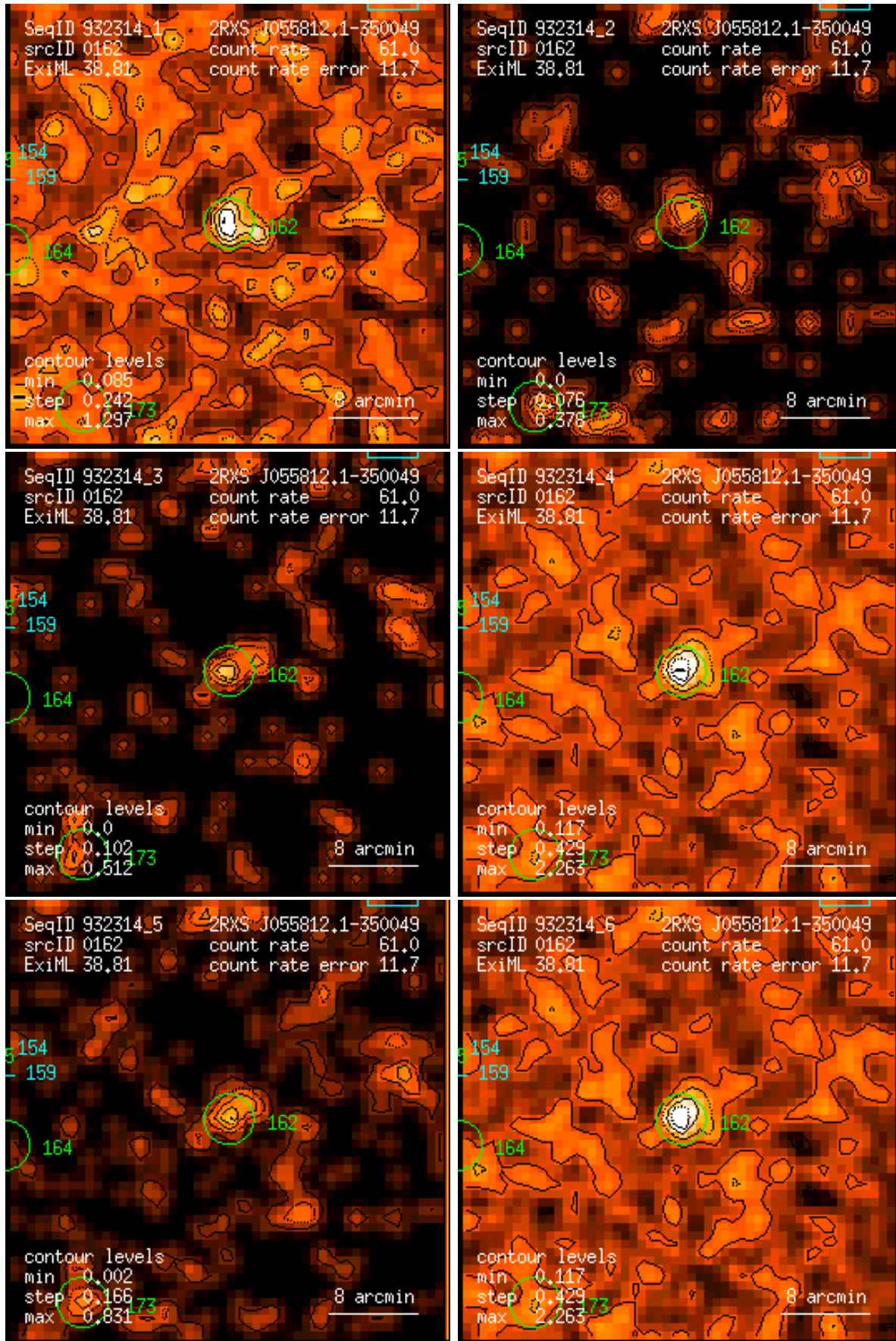
Figure 162: RASS 932314: detection 0162: band rate images, Gaussian filter: (1) PSPC channels 11 – 41, (2) 52 – 90, (3) 91 – 201, (4) 11 – 235, (5) 52 – 201, (6) 11 – 201. Broad band rates in counts/ks. Band rate contour levels in counts/ks/arcmin 2 .
