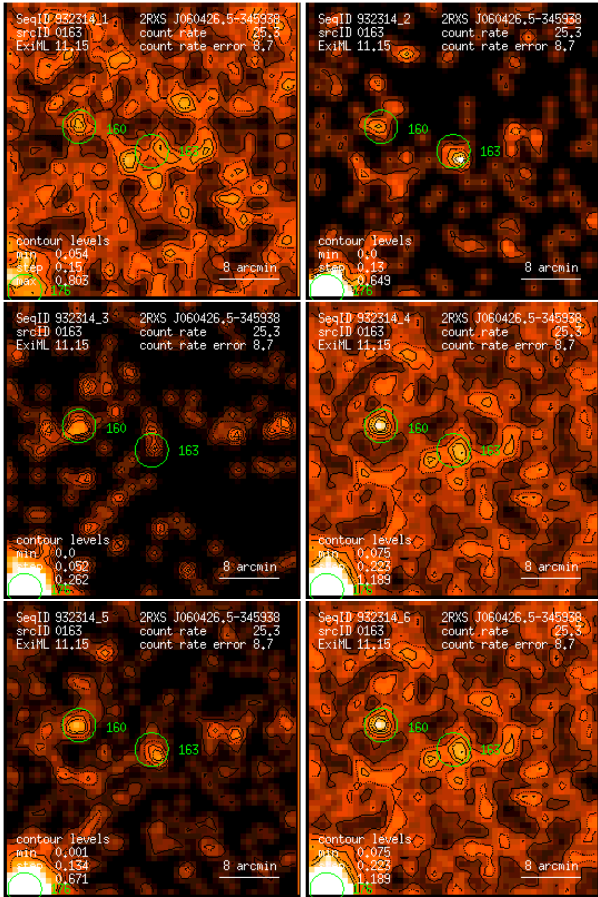
Figure 163: RASS 932314: detection 0163: band rate images, Gaussian filter: (1) PSPC channels 11 – 41, (2) 52 – 90, (3) 91 – 201, (4) 11 – 235, (5) 52 – 201, (6) 11 – 201. Broad band rates in counts/ks. Band rate contour levels in counts/ks/arcmin 2 .
