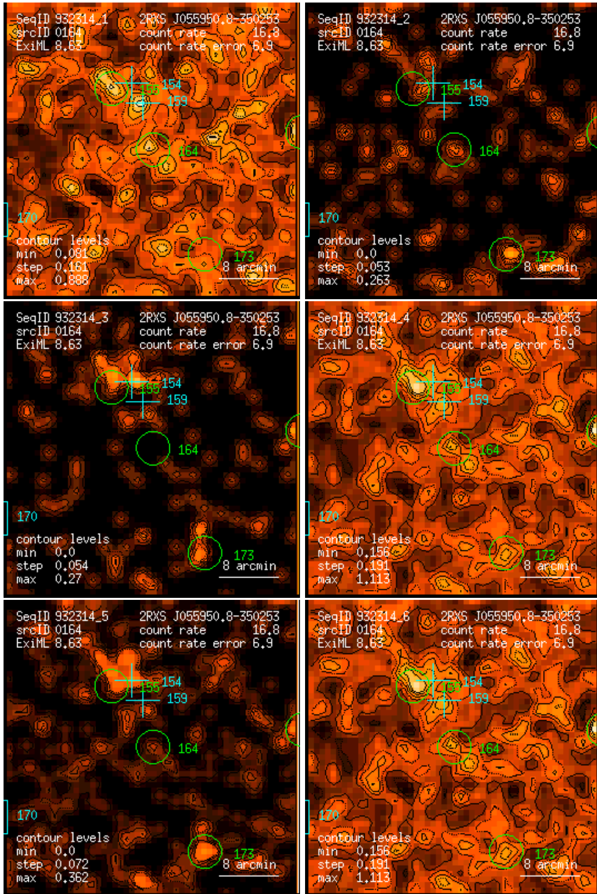
Figure 164: RASS 932314: detection 0164: band rate images, Gaussian filter: (1) PSPC channels 11 – 41, (2) 52 – 90, (3) 91 – 201, (4) 11 – 235, (5) 52 – 201, (6) 11 – 201. Broad band rates in counts/ks. Band rate contour levels in counts/ks/arcmin 2 .
