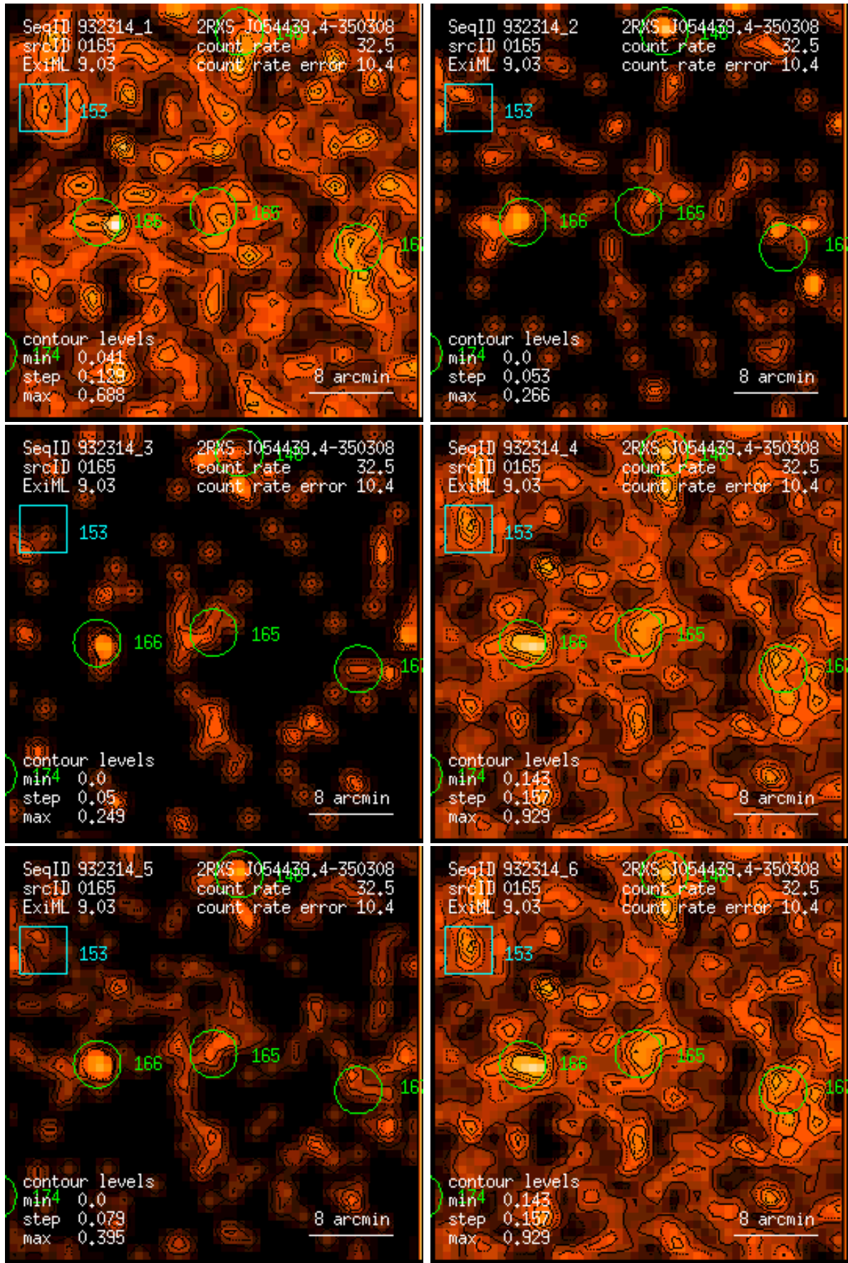
Figure 165: RASS 932314: detection 0165: band rate images, Gaussian filter: (1) PSPC channels 11 – 41, (2) 52 – 90, (3) 91 – 201, (4) 11 – 235, (5) 52 – 201, (6) 11 – 201. Broad band rates in counts/ks. Band rate contour levels in counts/ks/arcmin 2 .
