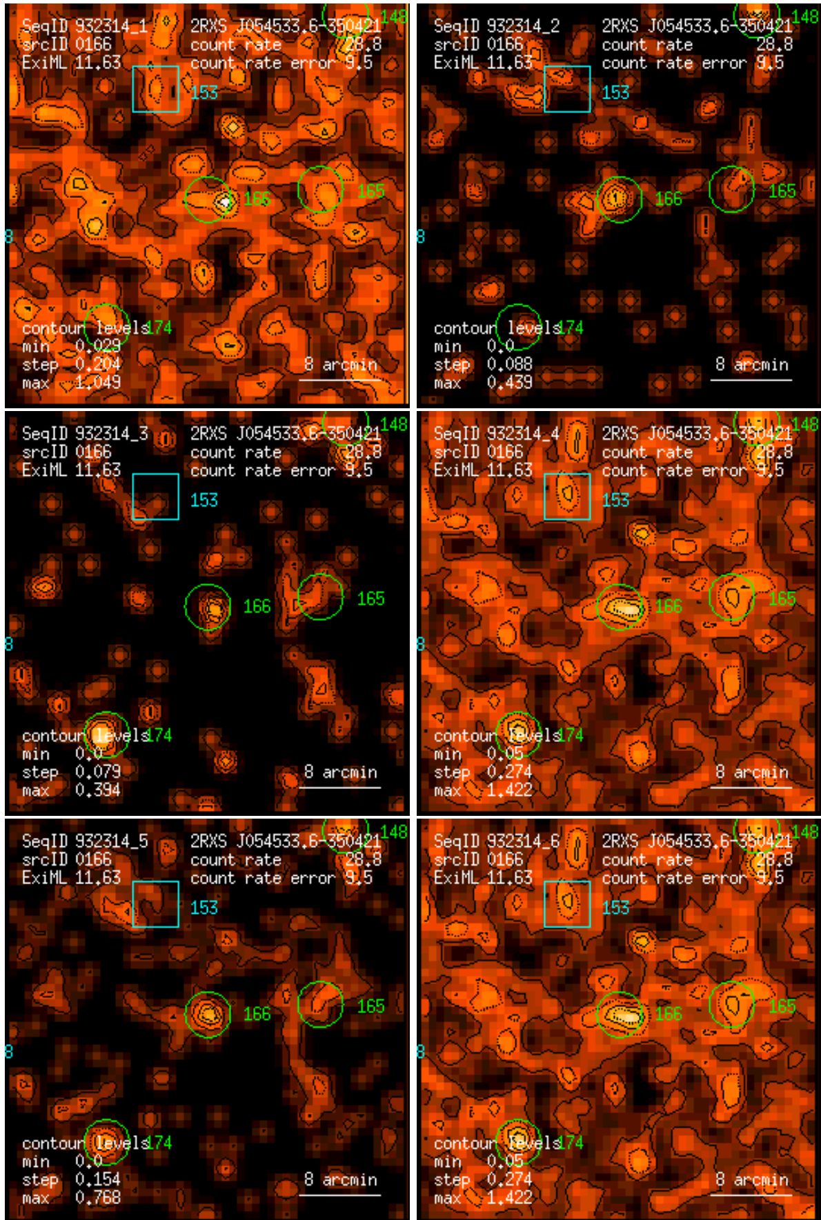
Figure 166: RASS 932314: detection 0166: band rate images, Gaussian filter: (1) PSPC channels 11 – 41, (2) 52 – 90, (3) 91 – 201, (4) 11 – 235, (5) 52 – 201, (6) 11 – 201. Broad band rates in counts/ks. Band rate contour levels in counts/ks/arcmin 2 .
