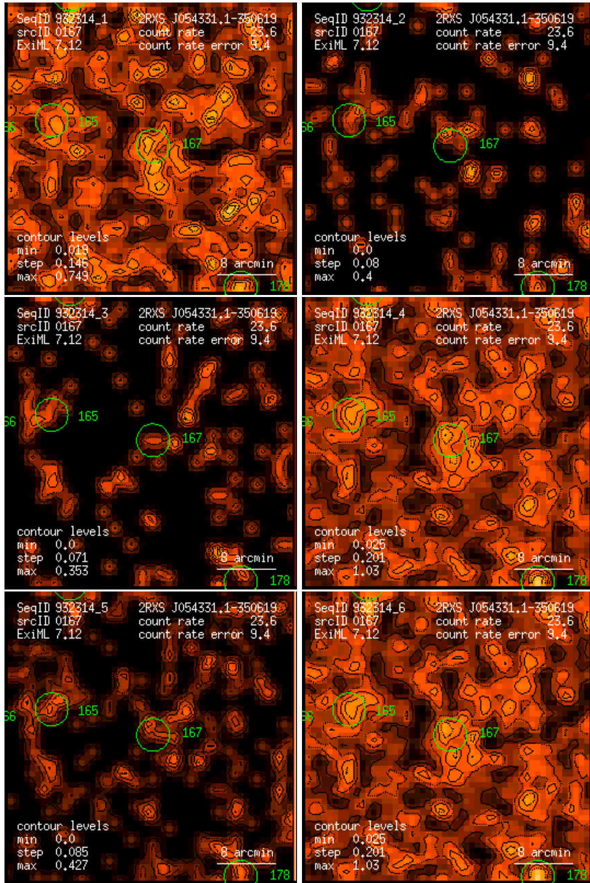
Figure 167: RASS 932314: detection 0167: band rate images, Gaussian filter: (1) PSPC channels 11 – 41, (2) 52 – 90, (3) 91 – 201, (4) 11 – 235, (5) 52 – 201, (6) 11 – 201. Broad band rates in counts/ks. Band rate contour levels in counts/ks/arcmin 2 .
