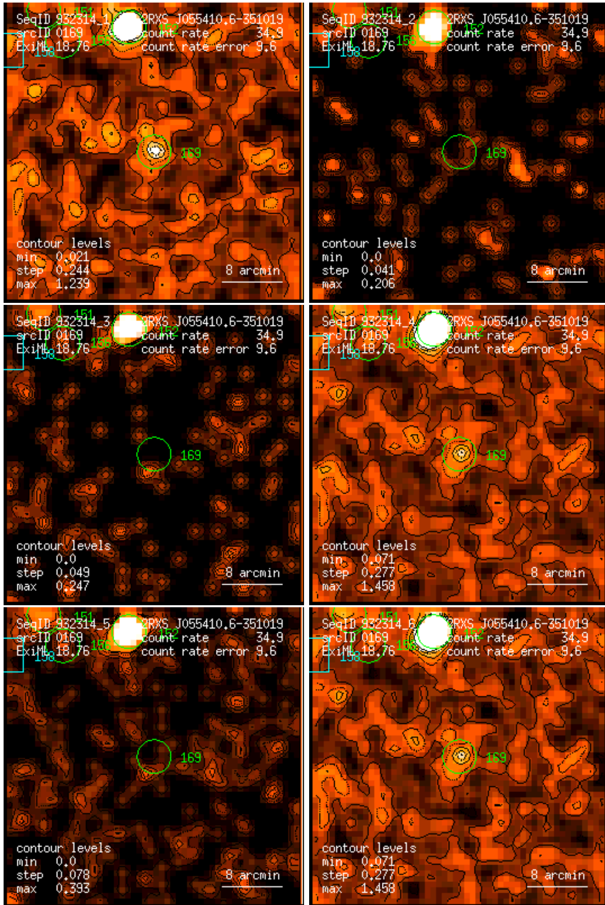
Figure 169: RASS 932314: detection 0169: band rate images, Gaussian filter: (1) PSPC channels 11 – 41, (2) 52 – 90, (3) 91 – 201, (4) 11 – 235, (5) 52 – 201, (6) 11 – 201. Broad band rates in counts/ks. Band rate contour levels in counts/ks/arcmin 2 .
