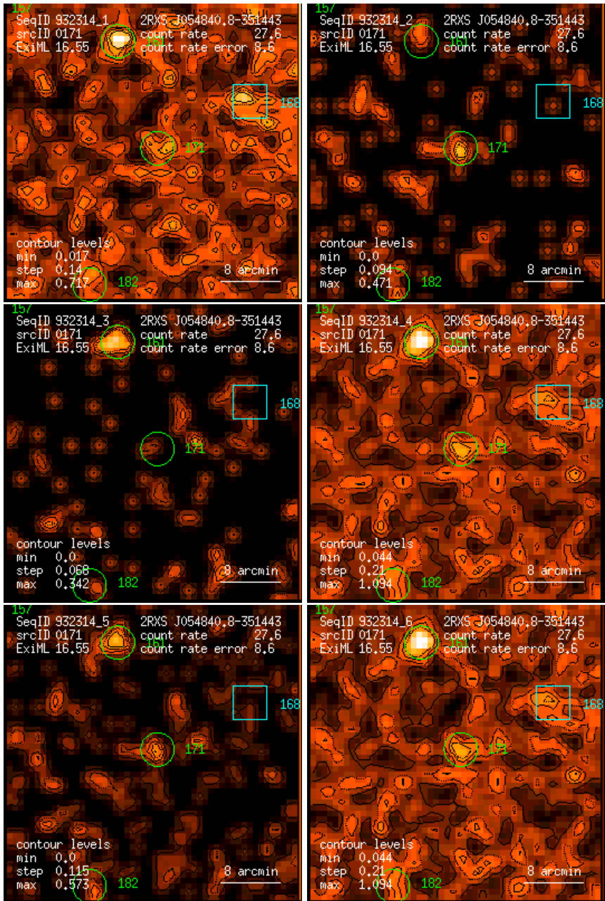
Figure 171: RASS 932314: detection 0171: band rate images, Gaussian filter: (1) PSPC channels 11 – 41, (2) 52 – 90, (3) 91 – 201, (4) 11 – 235, (5) 52 – 201, (6) 11 – 201. Broad band rates in counts/ks. Band rate contour levels in counts/ks/arcmin 2 .
