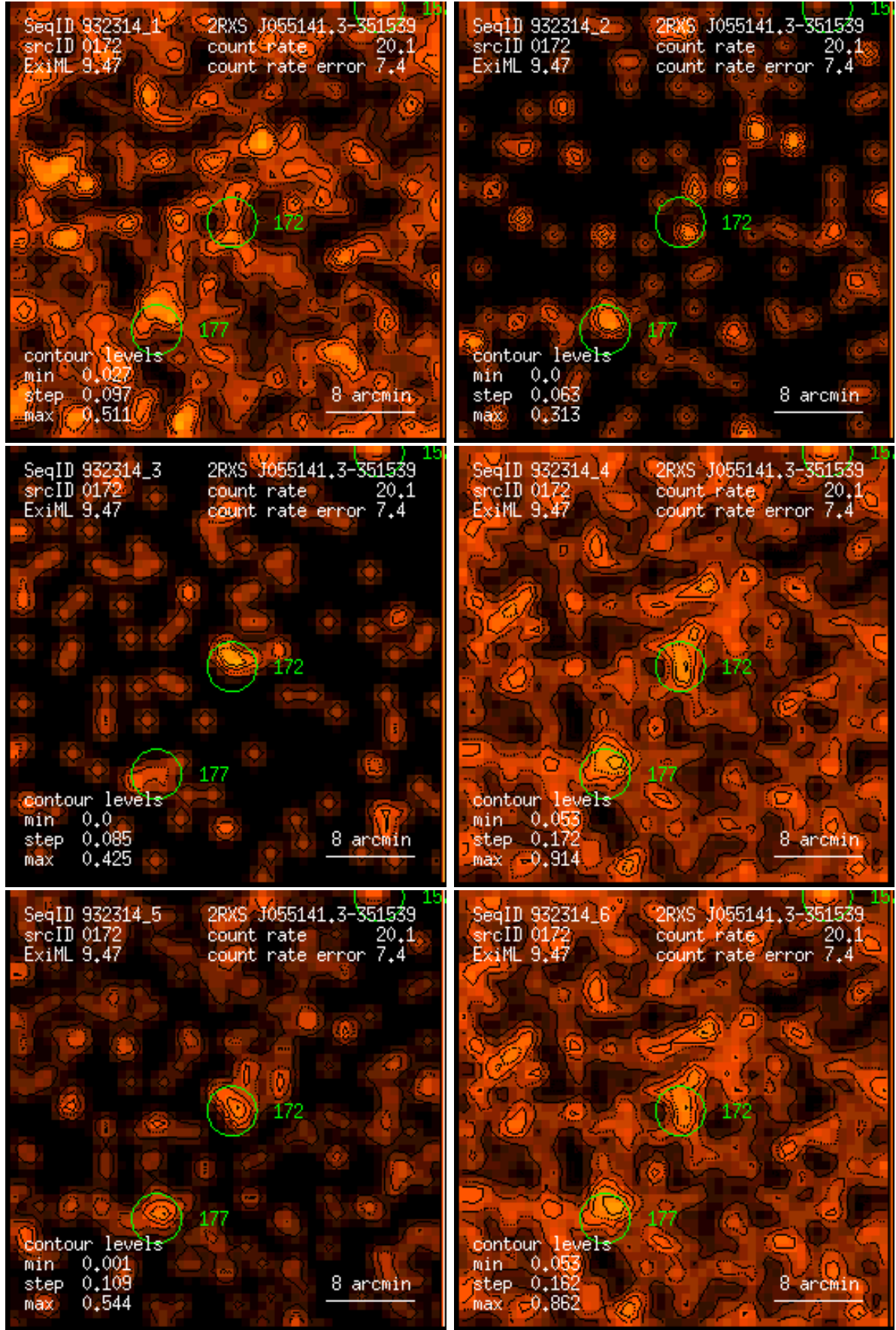
Figure 172: RASS 932314: detection 0172: band rate images, Gaussian filter: (1) PSPC channels 11 – 41, (2) 52 – 90, (3) 91 – 201, (4) 11 – 235, (5) 52 – 201, (6) 11 – 201. Broad band rates in counts/ks. Band rate contour levels in counts/ks/arcmin 2 .
