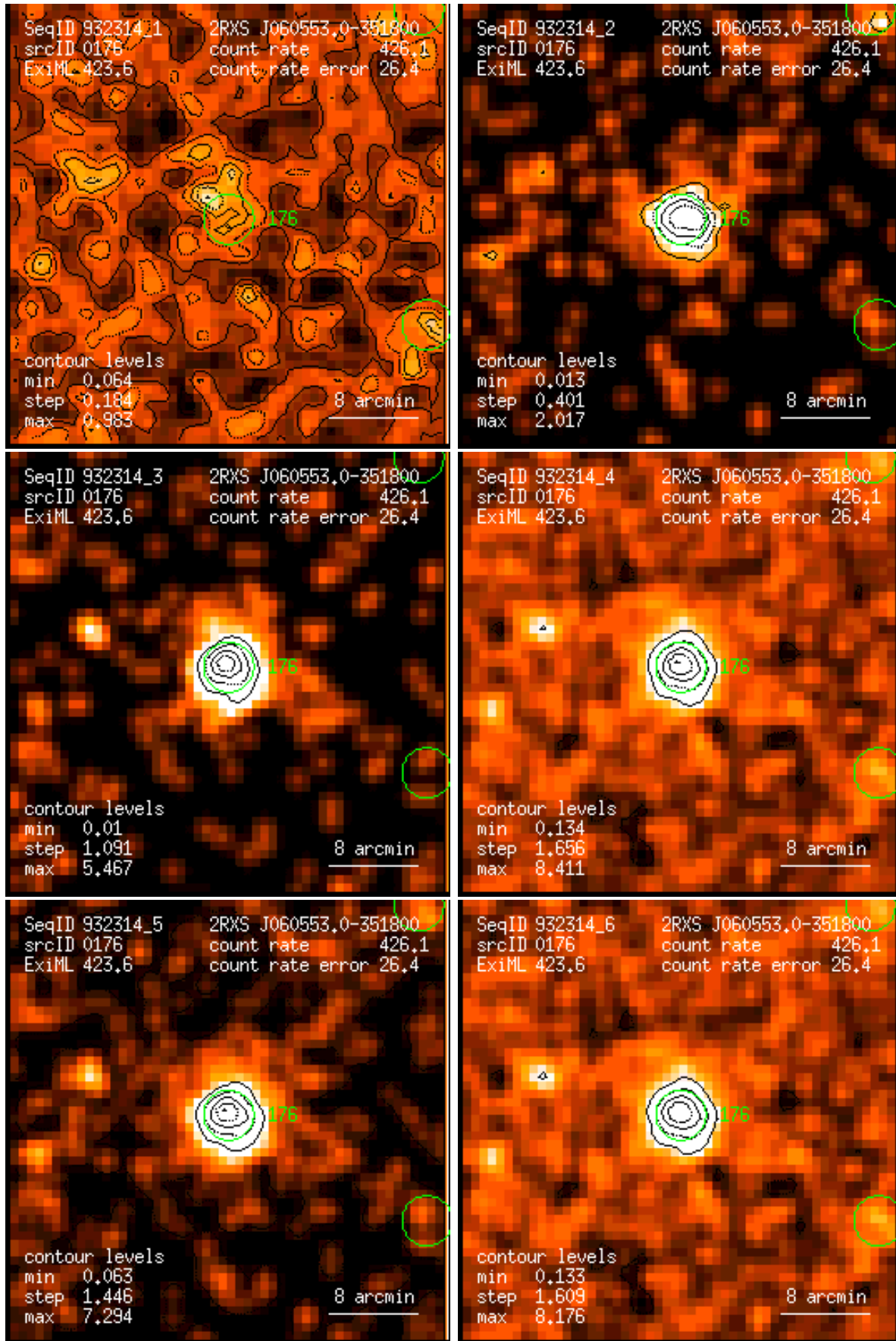
Figure 176: RASS 932314: detection 0176: band rate images, Gaussian filter: (1) PSPC channels 11 – 41, (2) 52 – 90, (3) 91 – 201, (4) 11 – 235, (5) 52 – 201, (6) 11 – 201. Broad band rates in counts/ks. Band rate contour levels in counts/ks/arcmin 2 .
