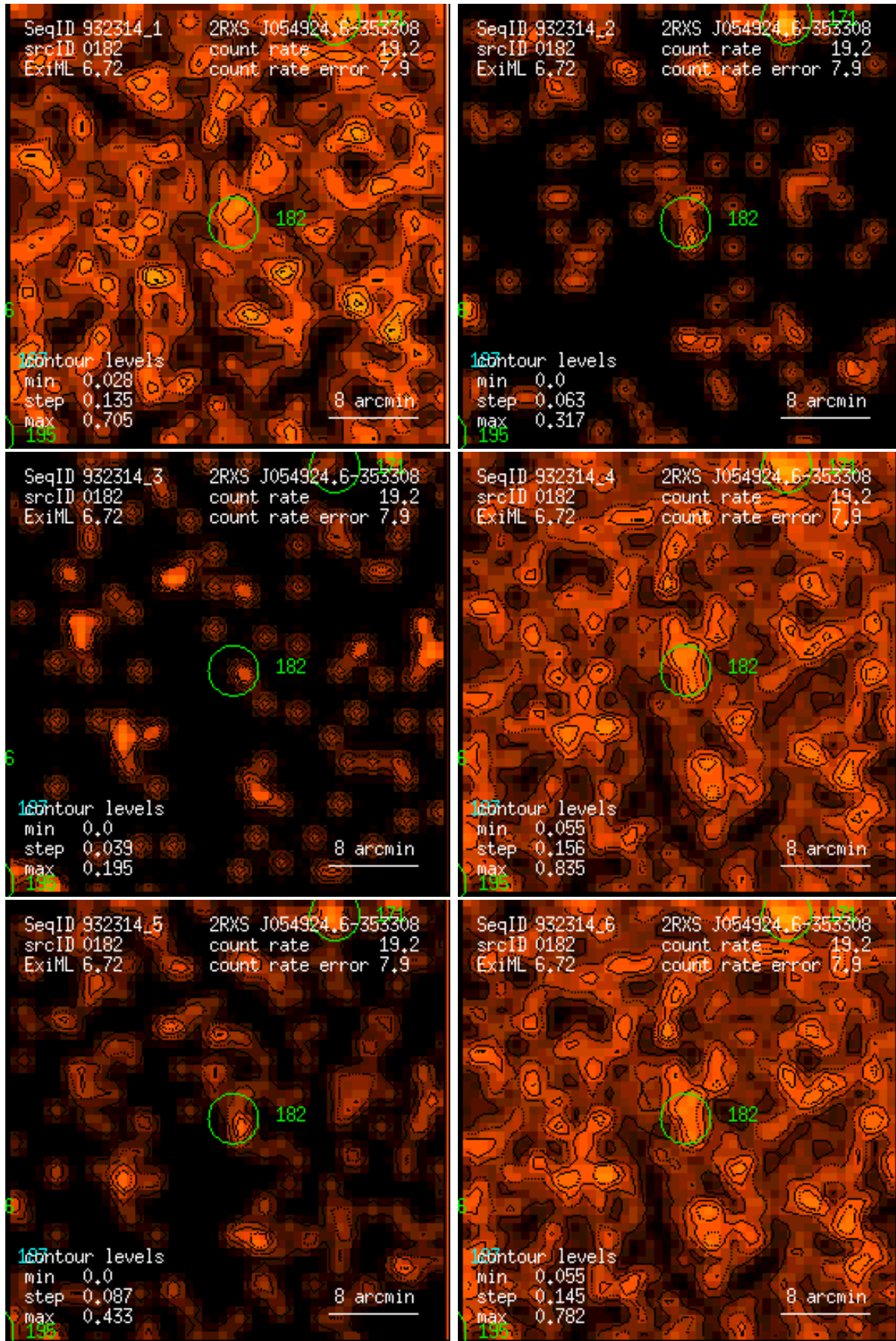
Figure 182: RASS 932314: detection 0182: band rate images, Gaussian filter: (1) PSPC channels 11 – 41, (2) 52 – 90, (3) 91 – 201, (4) 11 – 235, (5) 52 – 201, (6) 11 – 201. Broad band rates in counts/ks. Band rate contour levels in counts/ks/arcmin 2 .
