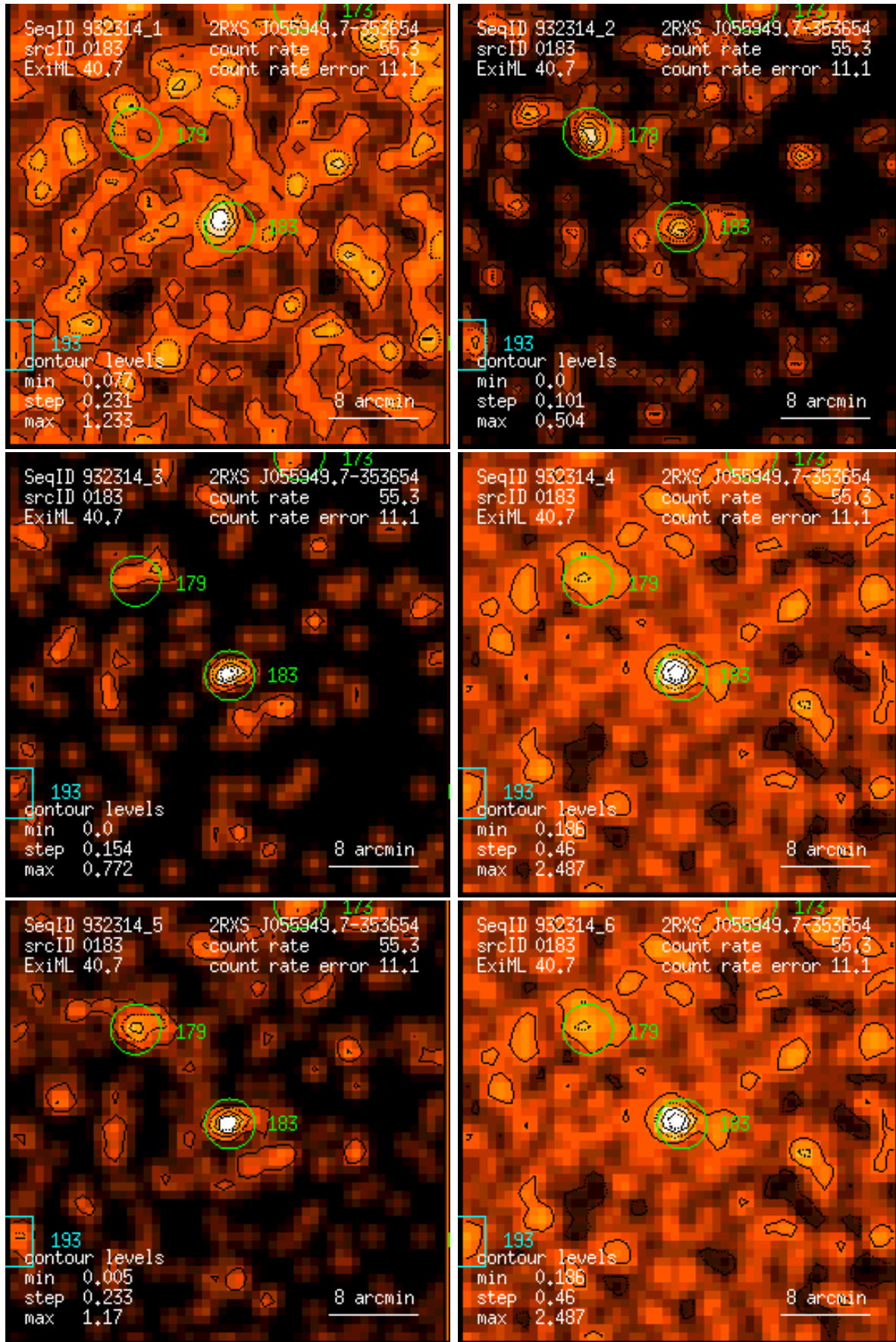
Figure 183: RASS 932314: detection 0183: band rate images, Gaussian filter: (1) PSPC channels 11 – 41, (2) 52 – 90, (3) 91 – 201, (4) 11 – 235, (5) 52 – 201, (6) 11 – 201. Broad band rates in counts/ks. Band rate contour levels in counts/ks/arcmin 2 .
