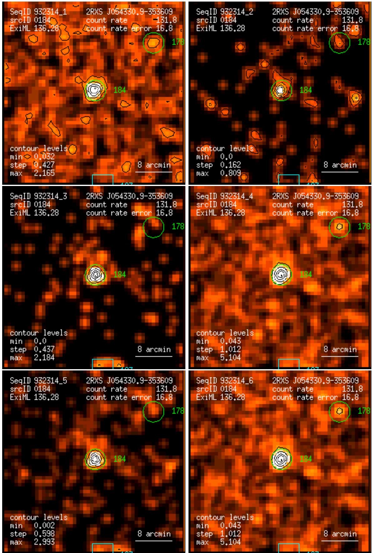
Figure 184: RASS 932314: detection 0184: band rate images, Gaussian filter: (1) PSPC channels 11 – 41, (2) 52 – 90, (3) 91 – 201, (4) 11 – 235, (5) 52 – 201, (6) 11 – 201. Broad band rates in counts/ks. Band rate contour levels in counts/ks/arcmin 2 .
