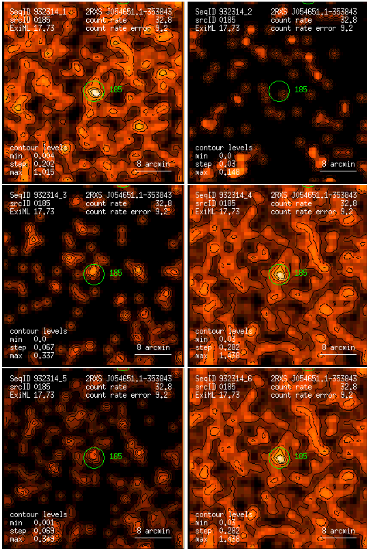
Figure 185: RASS 932314: detection 0185: band rate images, Gaussian filter: (1) PSPC channels 11 – 41, (2) 52 – 90, (3) 91 – 201, (4) 11 – 235, (5) 52 – 201, (6) 11 – 201. Broad band rates in counts/ks. Band rate contour levels in counts/ks/arcmin 2 .
