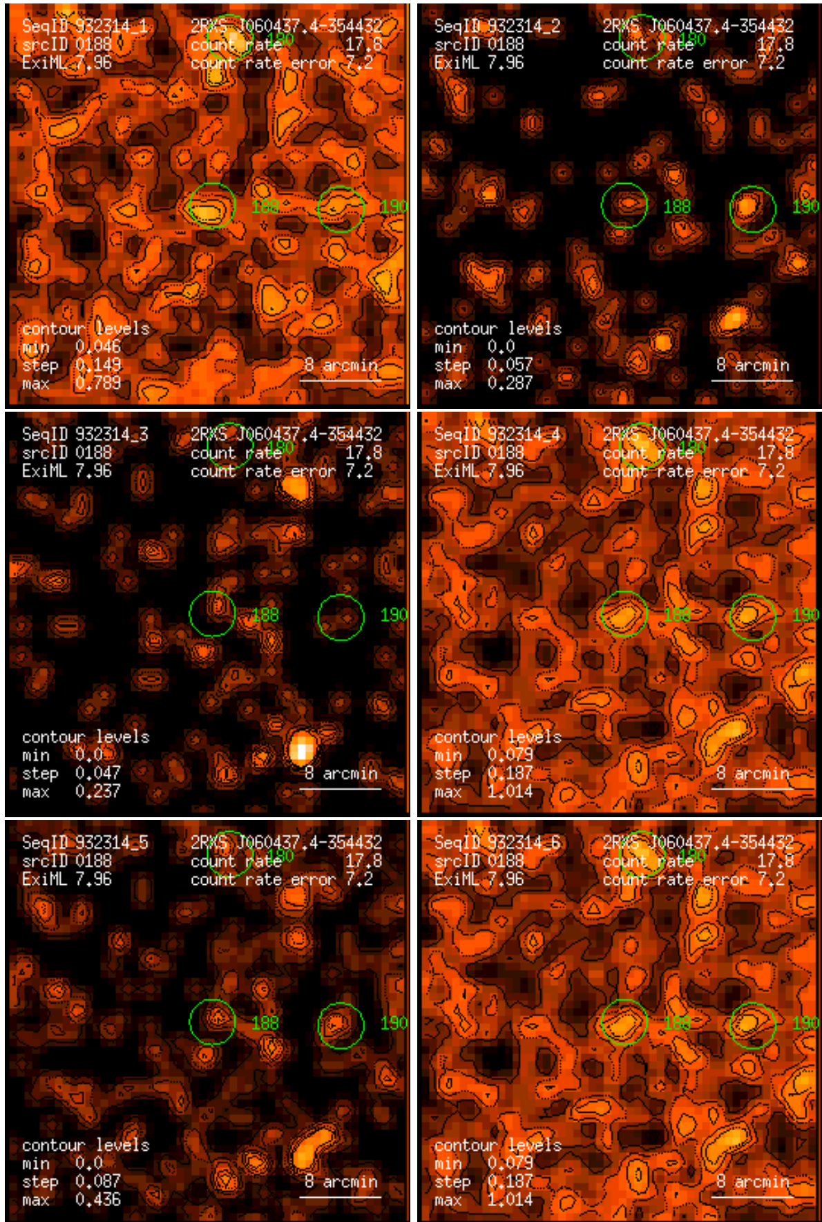
Figure 188: RASS 932314: detection 0188: band rate images, Gaussian filter: (1) PSPC channels 11 – 41, (2) 52 – 90, (3) 91 – 201, (4) 11 – 235, (5) 52 – 201, (6) 11 – 201. Broad band rates in counts/ks. Band rate contour levels in counts/ks/arcmin 2 .
