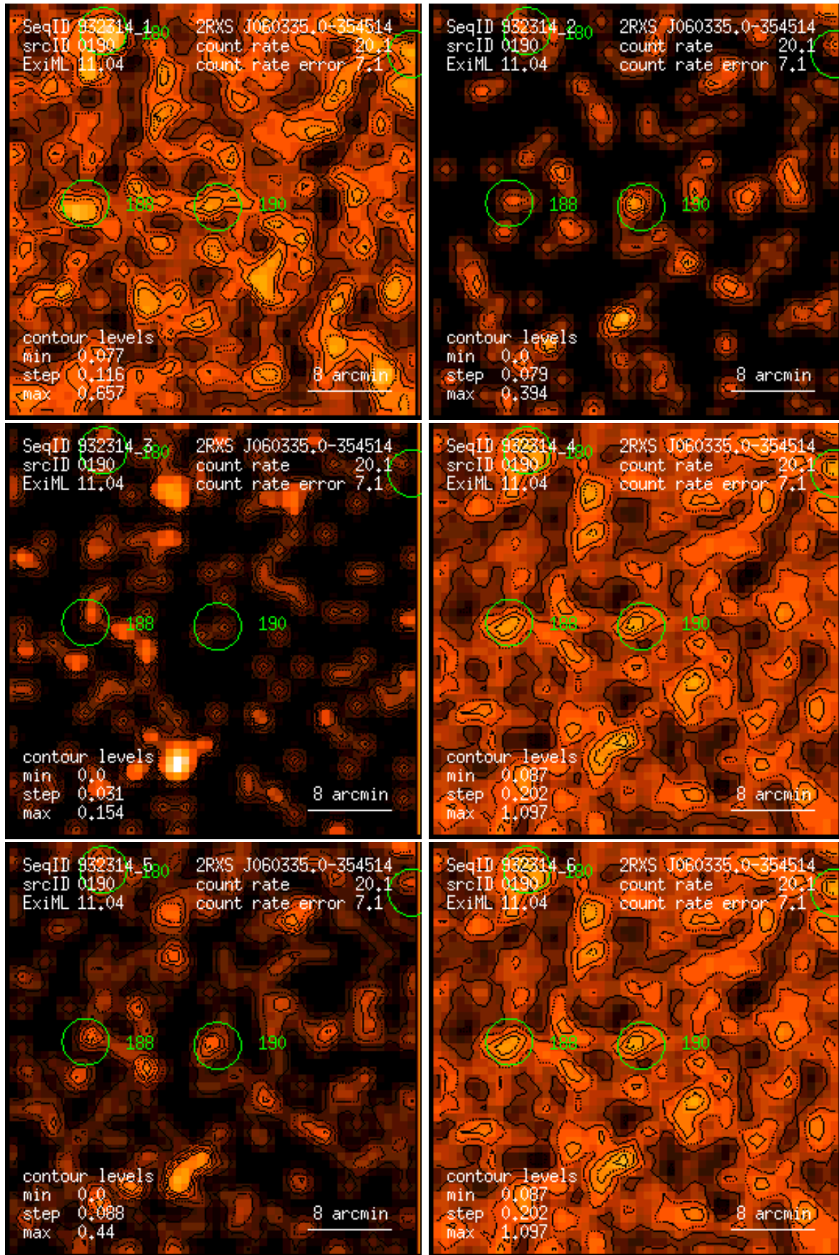
Figure 190: RASS 932314: detection 0190: band rate images, Gaussian filter: (1) PSPC channels 11 – 41, (2) 52 – 90, (3) 91 – 201, (4) 11 – 235, (5) 52 – 201, (6) 11 – 201. Broad band rates in counts/ks. Band rate contour levels in counts/ks/arcmin 2 .
