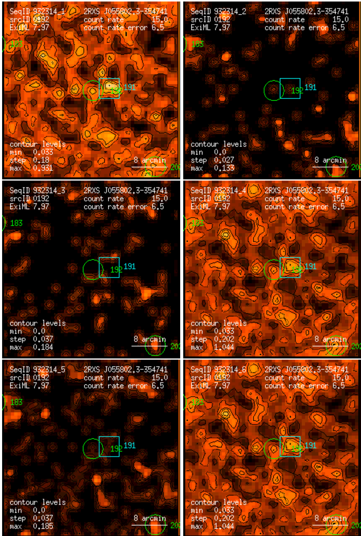
Figure 192: RASS 932314: detection 0192: band rate images, Gaussian filter: (1) PSPC channels 11 – 41, (2) 52 – 90, (3) 91 – 201, (4) 11 – 235, (5) 52 – 201, (6) 11 – 201. Broad band rates in counts/ks. Band rate contour levels in counts/ks/arcmin 2 .
