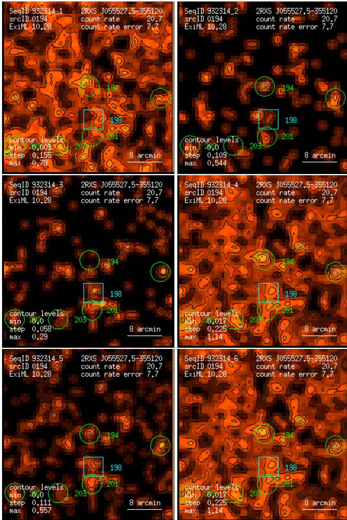
Figure 194: RASS 932314: detection 0194: band rate images, Gaussian filter: (1) PSPC channels 11 – 41, (2) 52 – 90, (3) 91 – 201, (4) 11 – 235, (5) 52 – 201, (6) 11 – 201. Broad band rates in counts/ks. Band rate contour levels in counts/ks/arcmin 2 .
