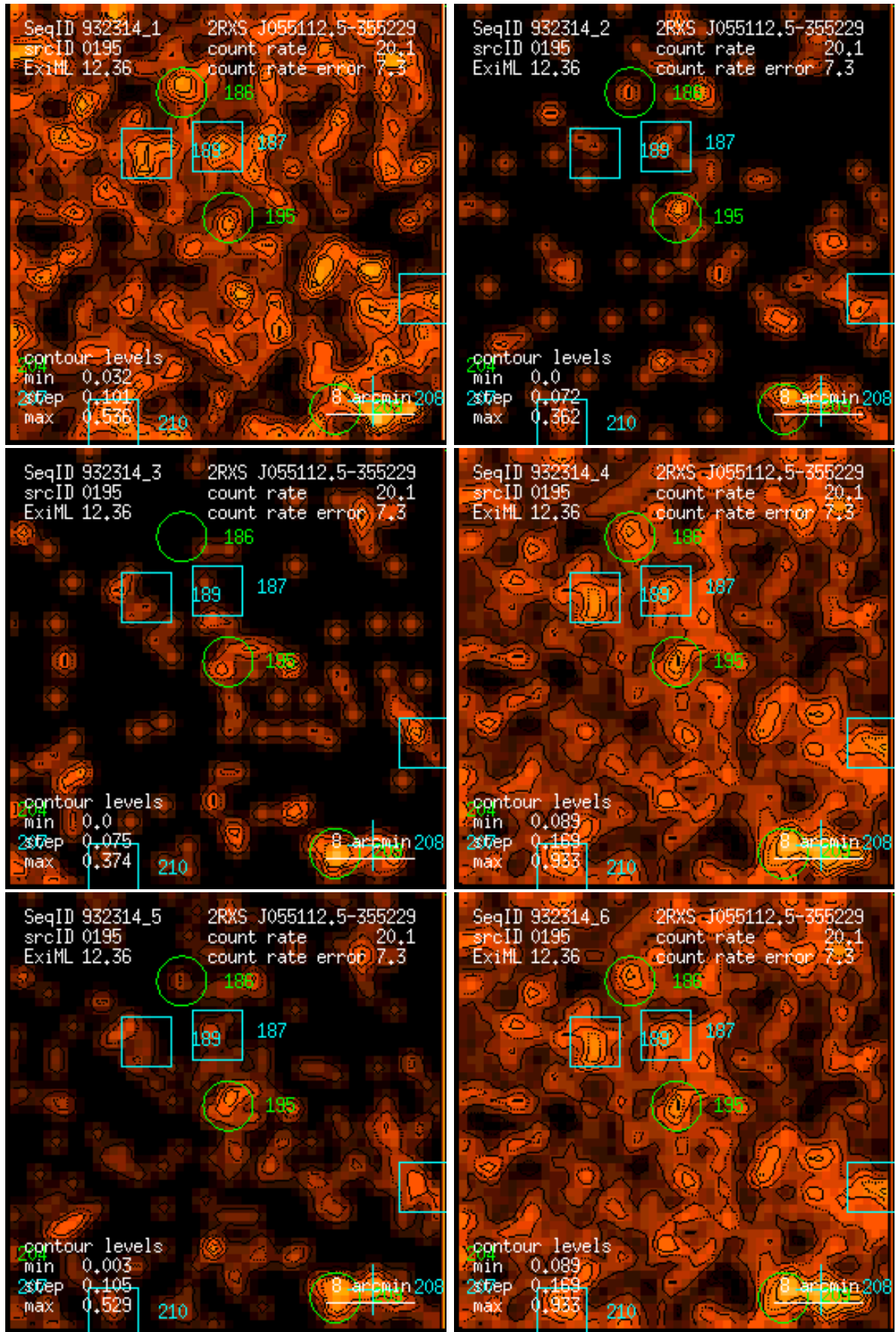
Figure 195: RASS 932314: detection 0195: band rate images, Gaussian filter: (1) PSPC channels 11 – 41, (2) 52 – 90, (3) 91 – 201, (4) 11 – 235, (5) 52 – 201, (6) 11 – 201. Broad band rates in counts/ks. Band rate contour levels in counts/ks/arcmin 2 .
