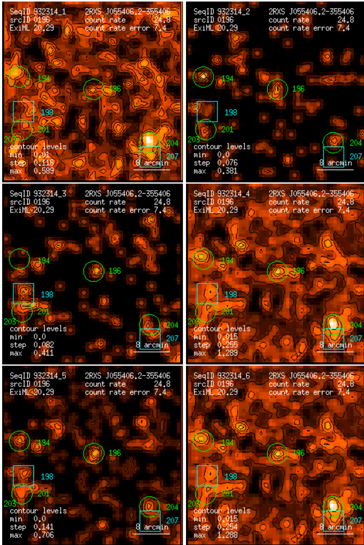
Figure 196: RASS 932314: detection 0196: band rate images, Gaussian filter: (1) PSPC channels 11 – 41, (2) 52 – 90, (3) 91 – 201, (4) 11 – 235, (5) 52 – 201, (6) 11 – 201. Broad band rates in counts/ks. Band rate contour levels in counts/ks/arcmin 2 .
