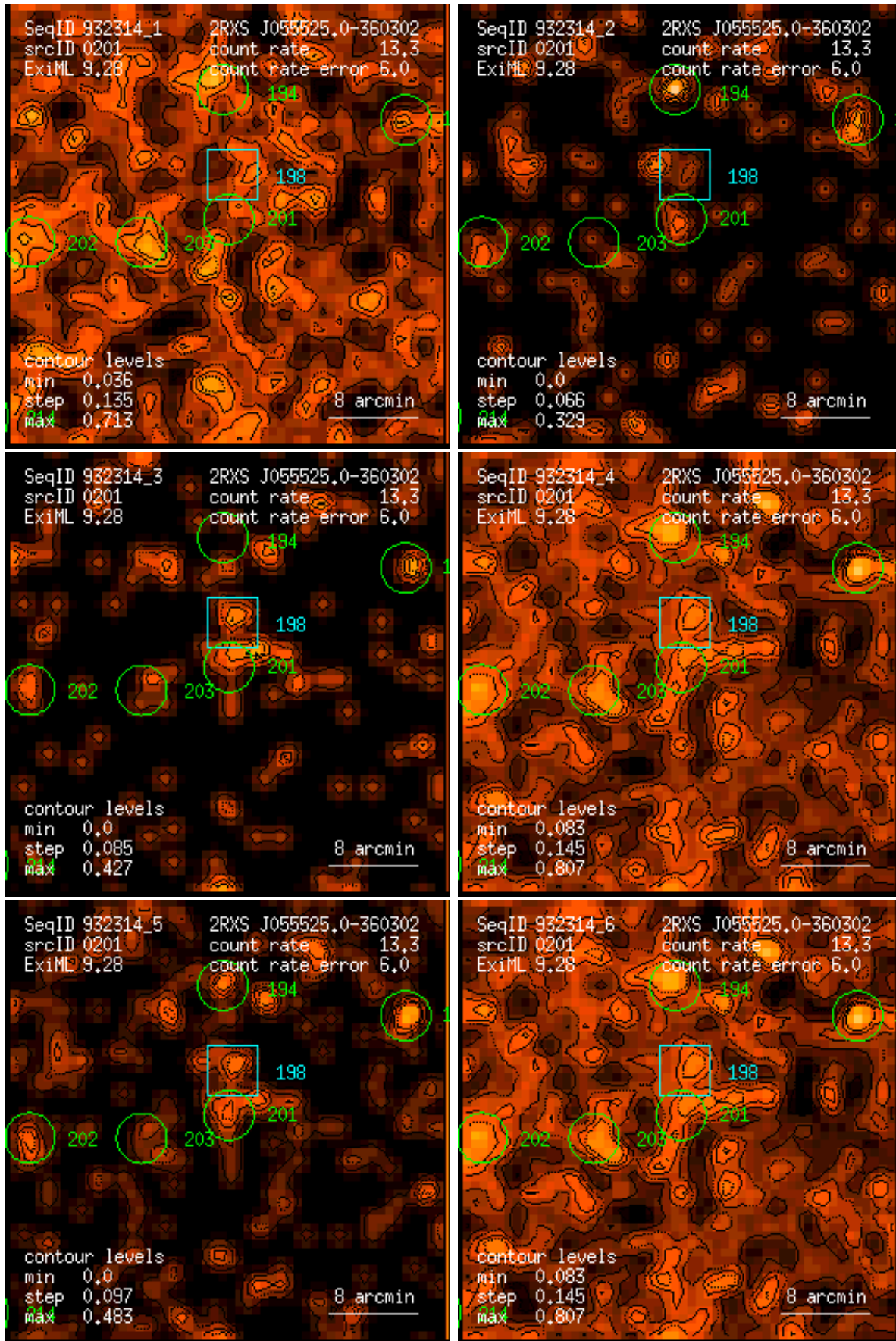
Figure 201: RASS 932314: detection 0201: band rate images, Gaussian filter: (1) PSPC channels 11 – 41, (2) 52 – 90, (3) 91 – 201, (4) 11 – 235, (5) 52 – 201, (6) 11 – 201. Broad band rates in counts/ks. Band rate contour levels in counts/ks/arcmin 2 .
