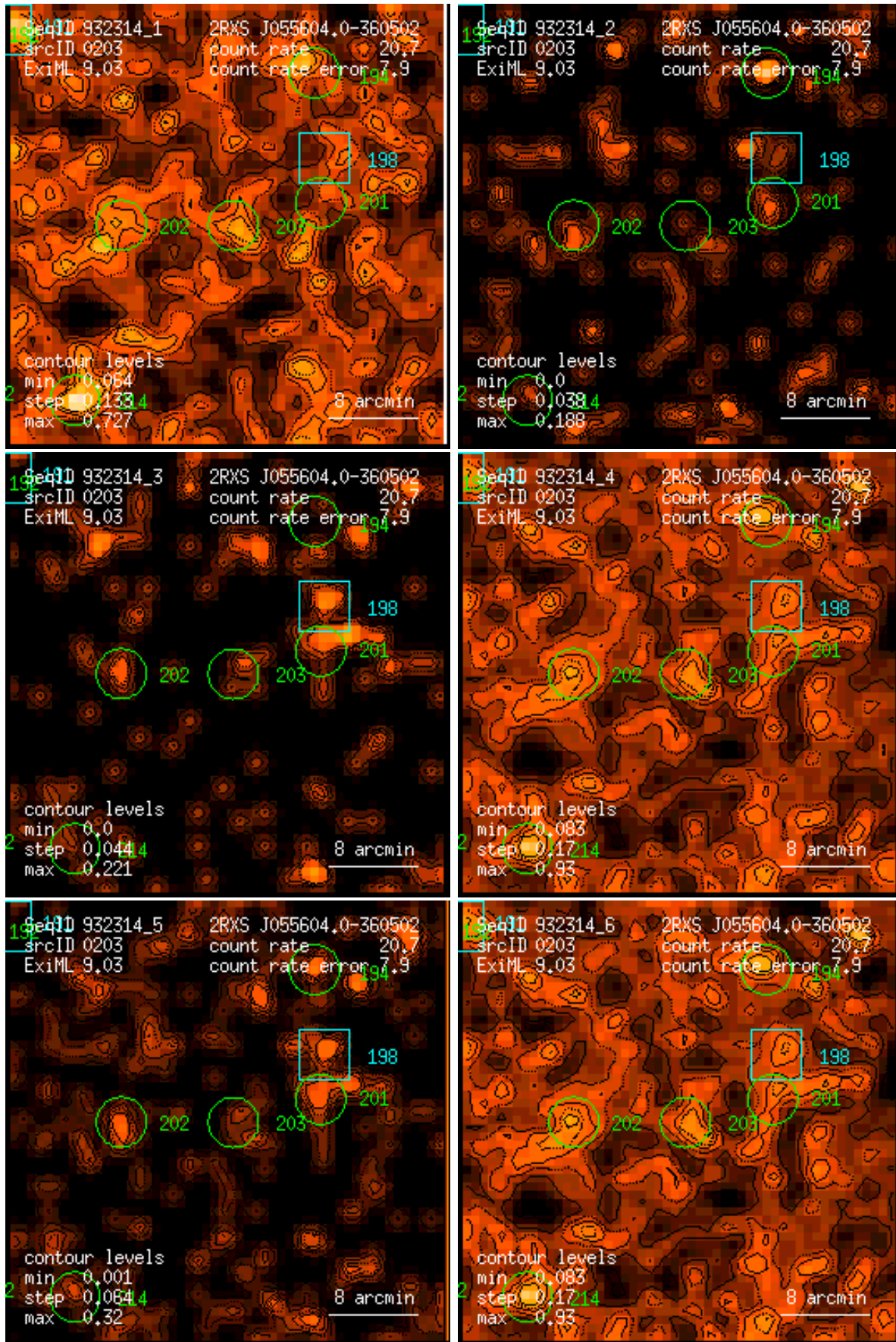
Figure 203: RASS 932314: detection 0203: band rate images, Gaussian filter: (1) PSPC channels 11 – 41, (2) 52 – 90, (3) 91 – 201, (4) 11 – 235, (5) 52 – 201, (6) 11 – 201. Broad band rates in counts/ks. Band rate contour levels in counts/ks/arcmin 2 .
