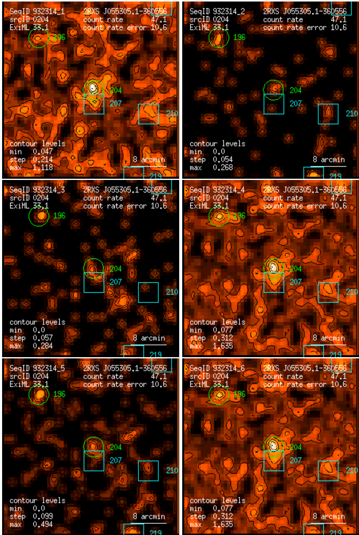
Figure 204: RASS 932314: detection 0204: band rate images, Gaussian filter: (1) PSPC channels 11 – 41, (2) 52 – 90, (3) 91 – 201, (4) 11 – 235, (5) 52 – 201, (6) 11 – 201. Broad band rates in counts/ks. Band rate contour levels in counts/ks/arcmin 2 .
