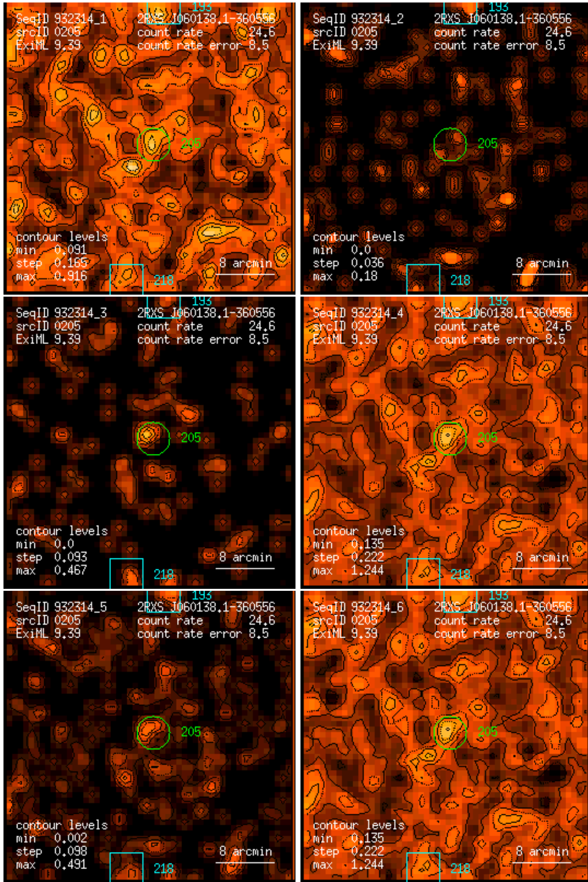
Figure 205: RASS 932314: detection 0205: band rate images, Gaussian filter: (1) PSPC channels 11 – 41, (2) 52 – 90, (3) 91 – 201, (4) 11 – 235, (5) 52 – 201, (6) 11 – 201. Broad band rates in counts/ks. Band rate contour levels in counts/ks/arcmin 2 .
