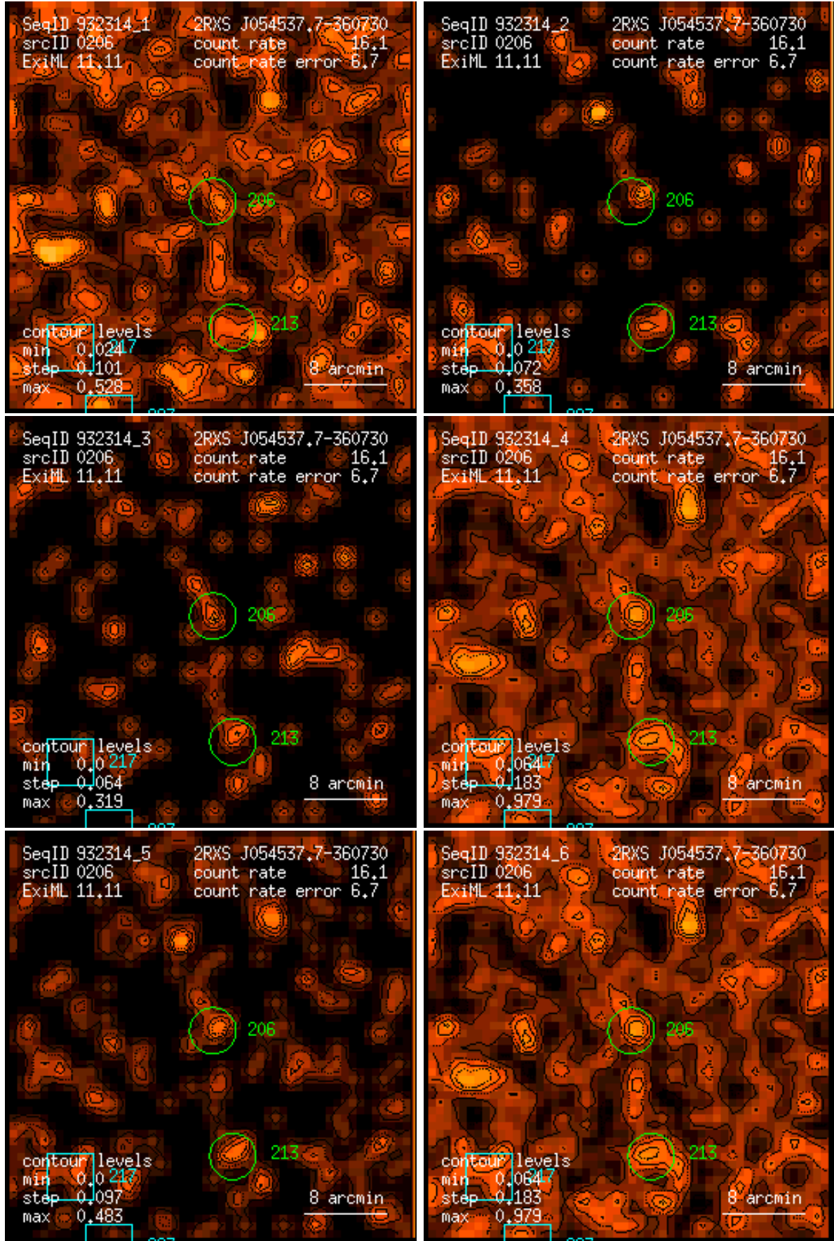
Figure 206: RASS 932314: detection 0206: band rate images, Gaussian filter: (1) PSPC channels 11 – 41, (2) 52 – 90, (3) 91 – 201, (4) 11 – 235, (5) 52 – 201, (6) 11 – 201. Broad band rates in counts/ks. Band rate contour levels in counts/ks/arcmin 2 .
