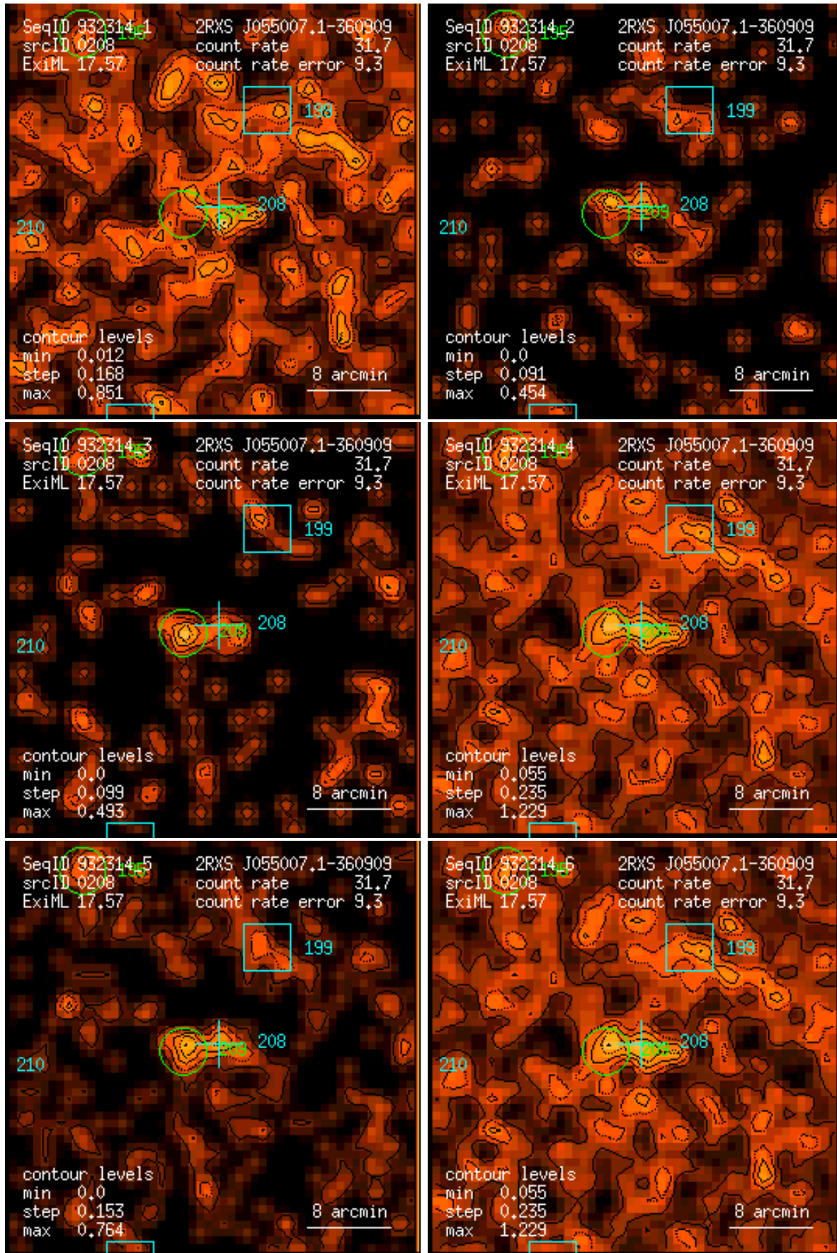
Figure 208: RASS 932314: detection 0208: band rate images, Gaussian filter: (1) PSPC channels 11 – 41, (2) 52 – 90, (3) 91 – 201, (4) 11 – 235, (5) 52 – 201, (6) 11 – 201. Broad band rates in counts/ks. Band rate contour levels in counts/ks/arcmin 2 .
