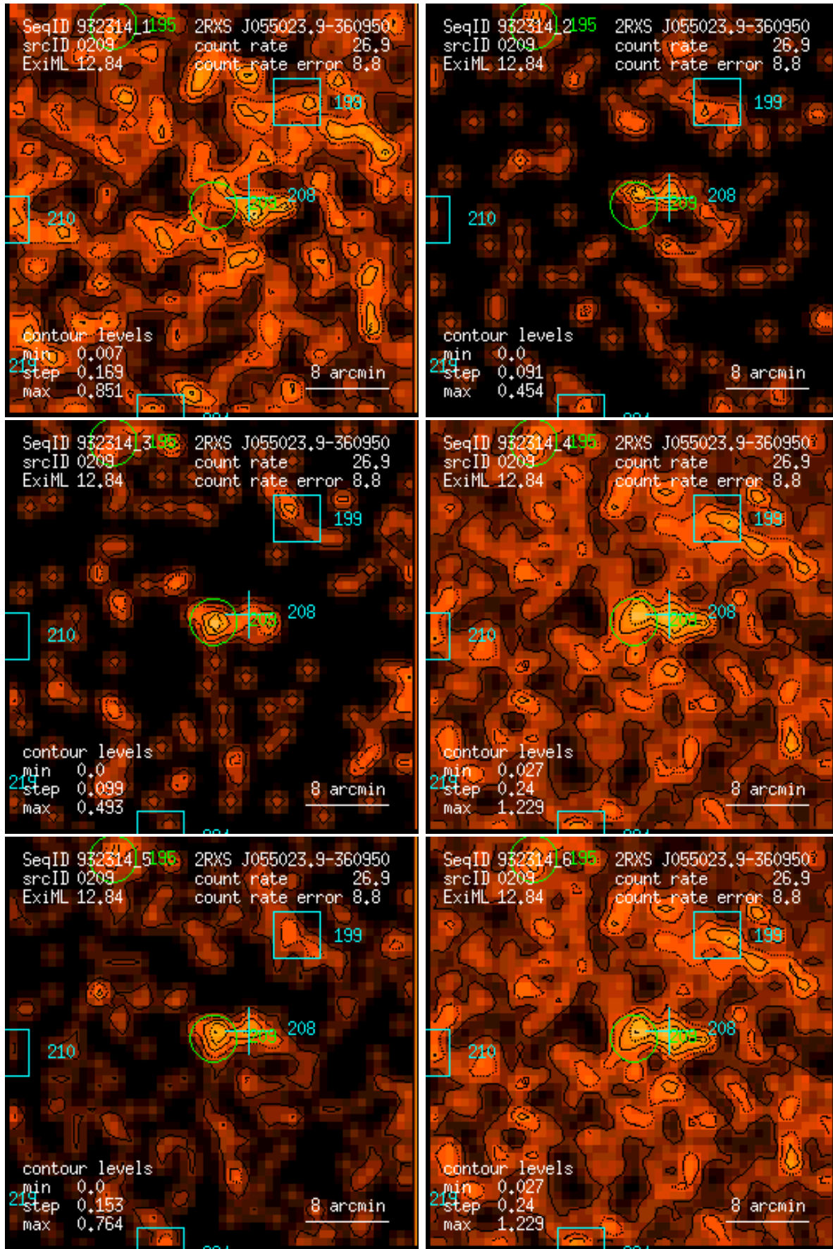
Figure 209: RASS 932314: detection 0209: band rate images, Gaussian filter: (1) PSPC channels 11 – 41, (2) 52 – 90, (3) 91 – 201, (4) 11 – 235, (5) 52 – 201, (6) 11 – 201. Broad band rates in counts/ks. Band rate contour levels in counts/ks/arcmin 2 .
