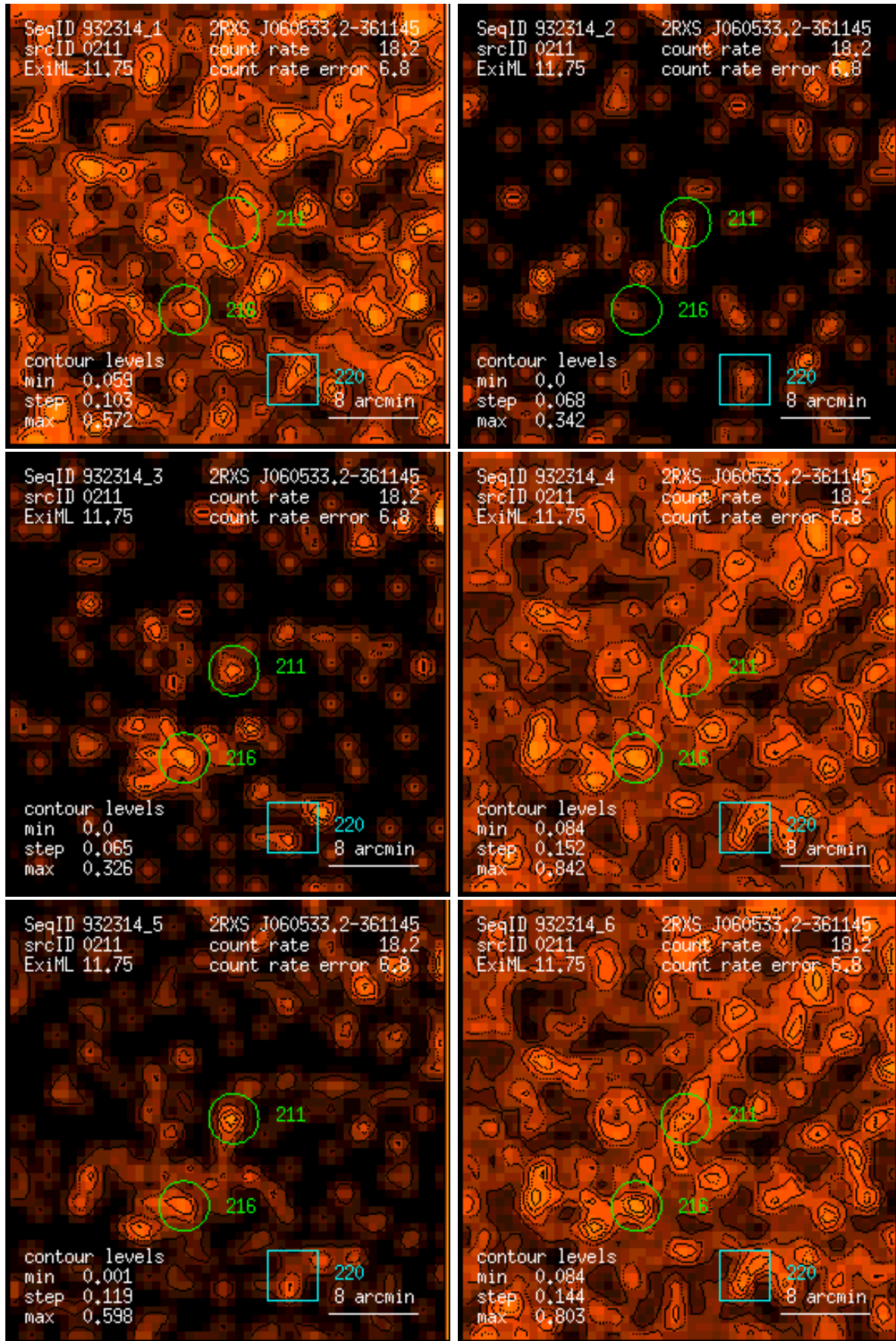
Figure 211: RASS 932314: detection 0211: band rate images, Gaussian filter: (1) PSPPC channels 11 – 41, (2) 52 – 90, (3) 91 – 201, (4) 11 – 235, (5) 52 – 201, (6) 11 – 201. Broad band rates in counts/ks. Band rate contour levels in counts/ks/arcmin 2 .
