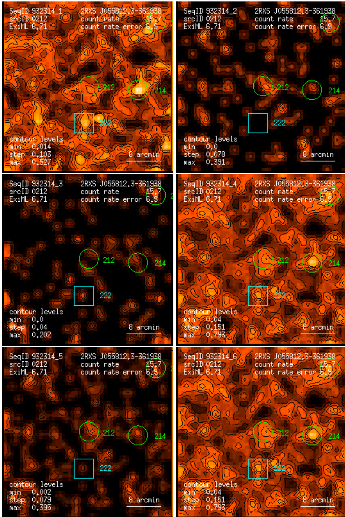
Figure 212: RASS 932314: detection 0212: band rate images, Gaussian filter: (1) PSPC channels 11 – 41, (2) 52 – 90, (3) 91 – 201, (4) 11 – 235, (5) 52 – 201, (6) 11 – 201. Broad band rates in counts/ks. Band rate contour levels in counts/ks/arcmin 2 .
