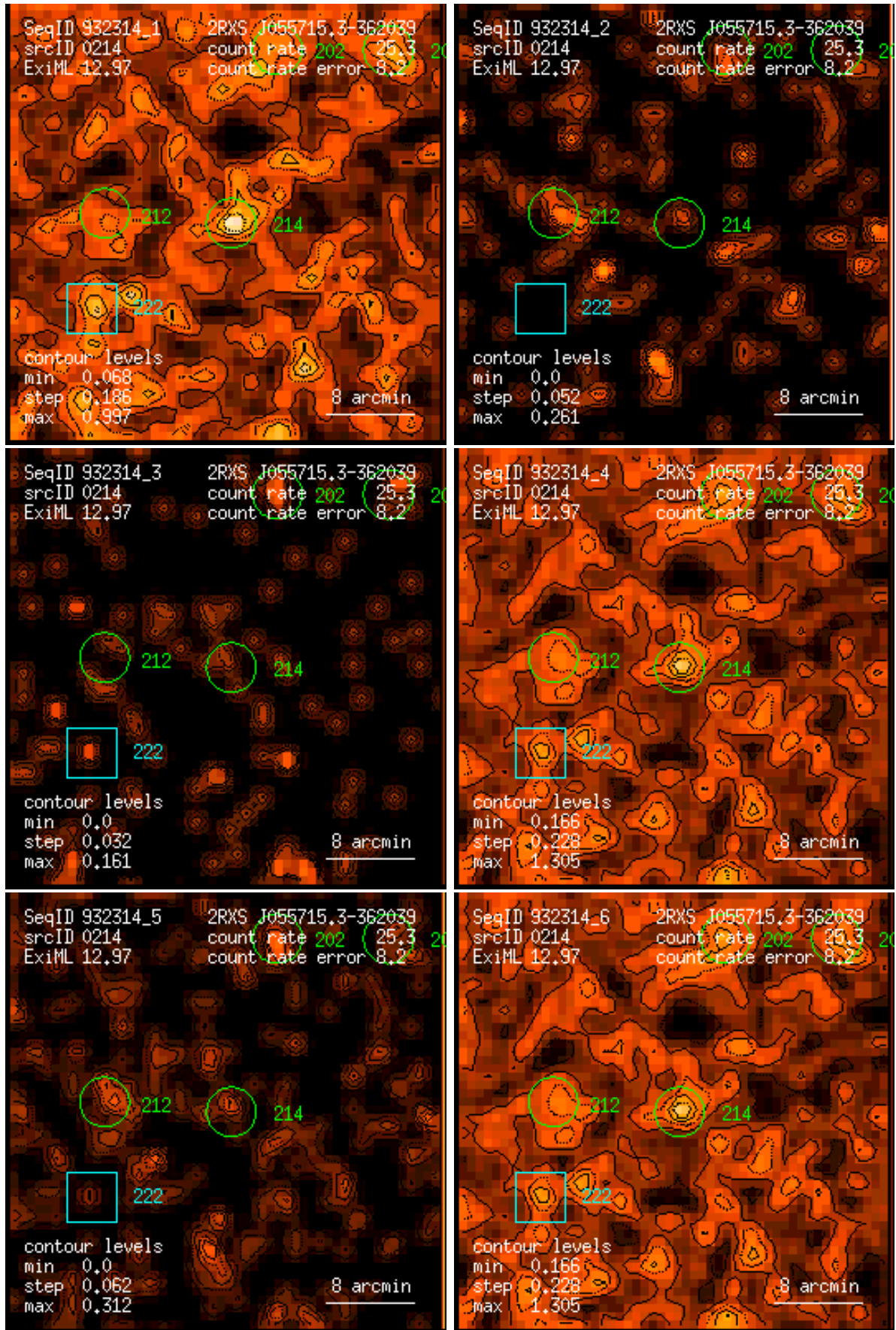
Figure 214: RASS 932314: detection 0214: band rate images, Gaussian filter: (1) PSPC channels 11 – 41, (2) 52 – 90, (3) 91 – 201, (4) 11 – 235, (5) 52 – 201, (6) 11 – 201. Broad band rates in counts/ks. Band rate contour levels in counts/ks/arcmin 2 .
