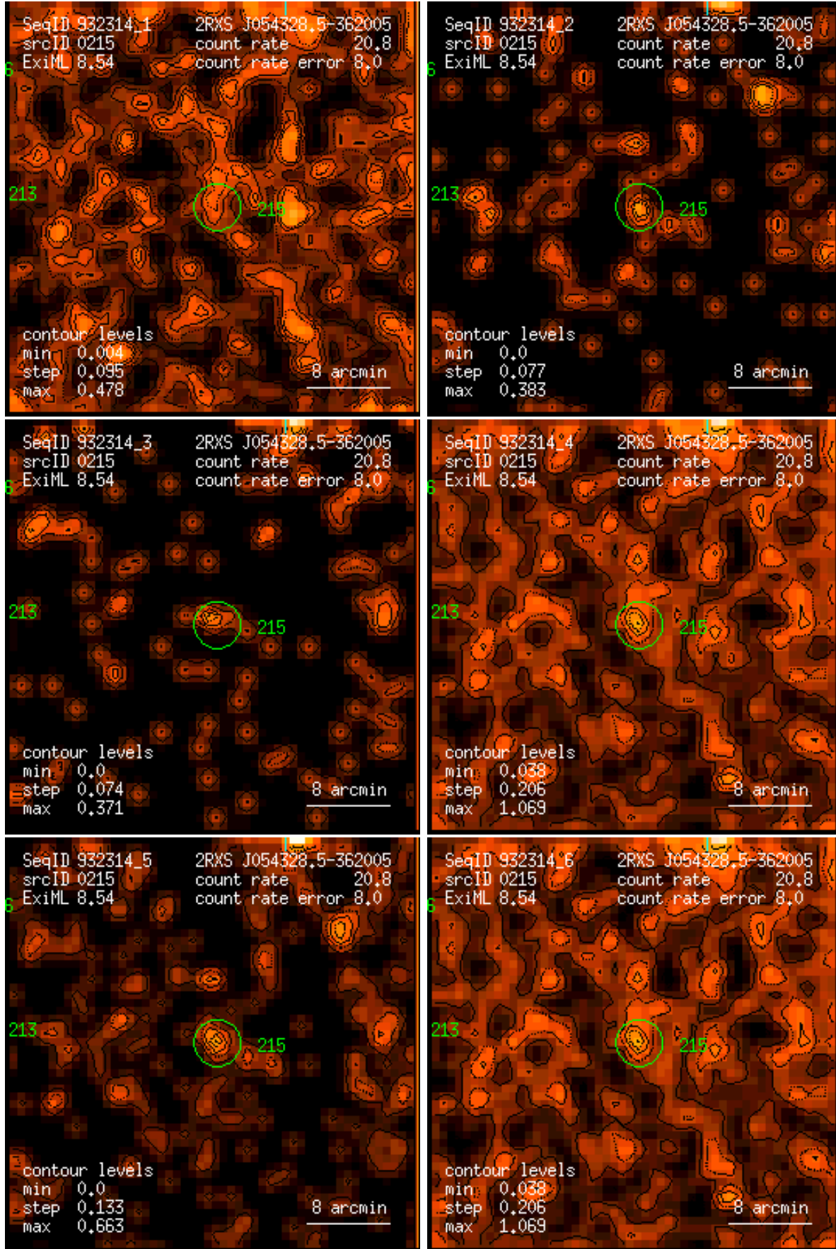
Figure 215: RASS 932314: detection 0215: band rate images, Gaussian filter: (1) PSPC channels 11 – 41, (2) 52 – 90, (3) 91 – 201, (4) 11 – 235, (5) 52 – 201, (6) 11 – 201. Broad band rates in counts/ks. Band rate contour levels in counts/ks/arcmin 2 .
