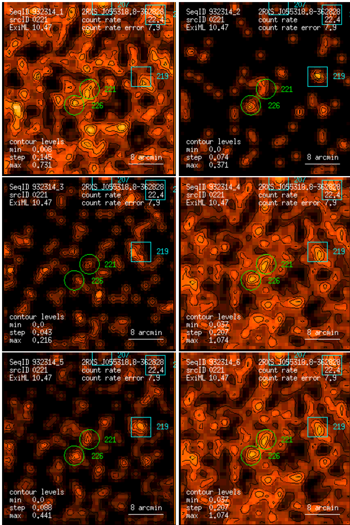
Figure 221: RASS 932314: detection 0221: band rate images, Gaussian filter: (1) PSPC channels 11 – 41, (2) 52 – 90, (3) 91 – 201, (4) 11 – 235, (5) 52 – 201, (6) 11 – 201. Broad band rates in counts/ks. Band rate contour levels in counts/ks/arcmin 2 .
