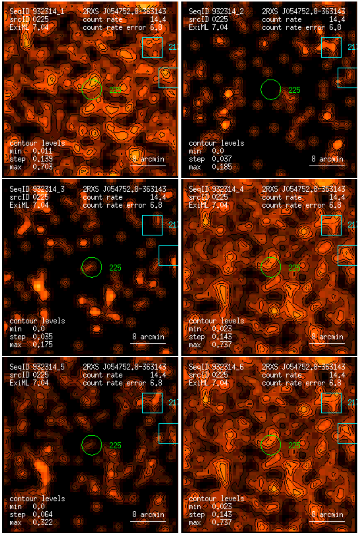
Figure 225: RASS 932314: detection 0225: band rate images, Gaussian filter: (1) PSPC channels 11 – 41, (2) 52 – 90, (3) 91 – 201, (4) 11 – 235, (5) 52 – 201, (6) 11 – 201. Broad band rates in counts/ks. Band rate contour levels in counts/ks/arcmin 2 .
