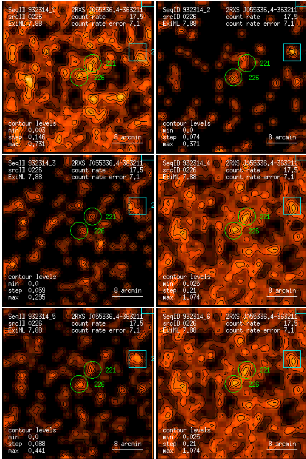
Figure 226: RASS 932314: detection 0226: band rate images, Gaussian filter: (1) PSPC channels 11 – 41, (2) 52 – 90, (3) 91 – 201, (4) 11 – 235, (5) 52 – 201, (6) 11 – 201. Broad band rates in counts/ks. Band rate contour levels in counts/ks/arcmin 2 .
