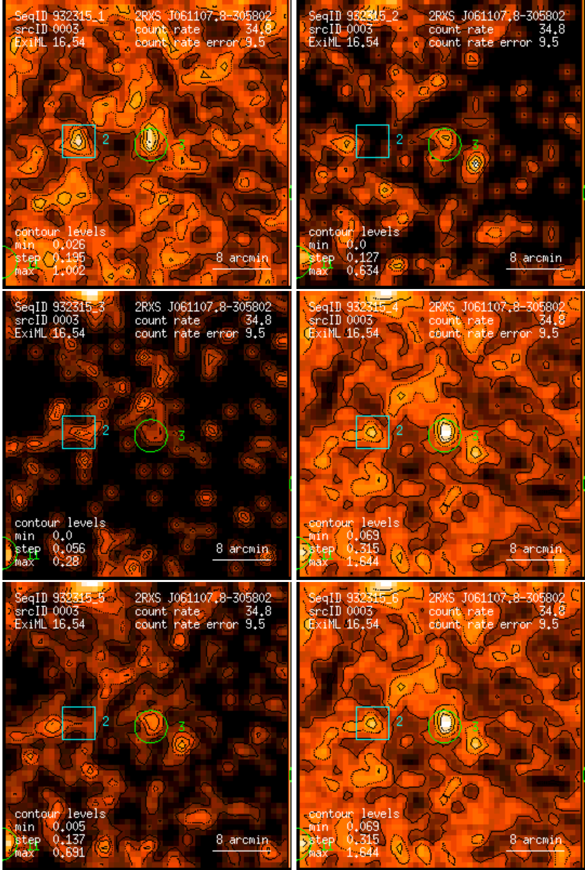
Figure 3: RASS 932315: detection 0003: band rate images, Gaussian filter: (1) PSPC channels 11 – 41, (2) 52 – 90, (3) 91 – 201, (4) 11 – 235, (5) 52 – 201, (6) 11 – 201. Broad band rates in counts/ks. Band rate contour levels in counts/ks/arcmin 2 .
