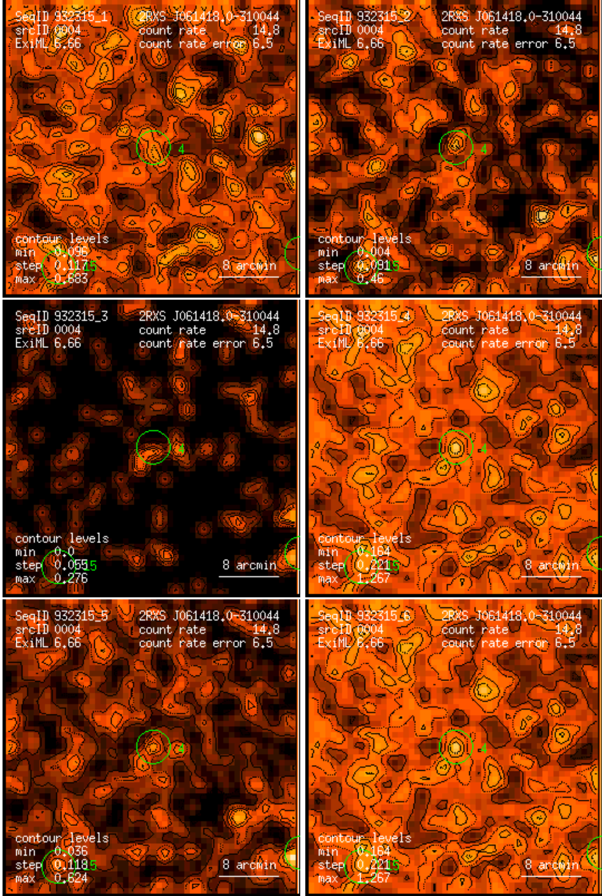
Figure 4: RASS 932315: detection 0004: band rate images, Gaussian filter: (1) PSPC channels 11 – 41, (2) 52 – 90, (3) 91 – 201, (4) 11 – 235, (5) 52 – 201, (6) 11 – 201. Broad band rates in counts/ks. Band rate contour levels in counts/ks/arcmin 2 .
