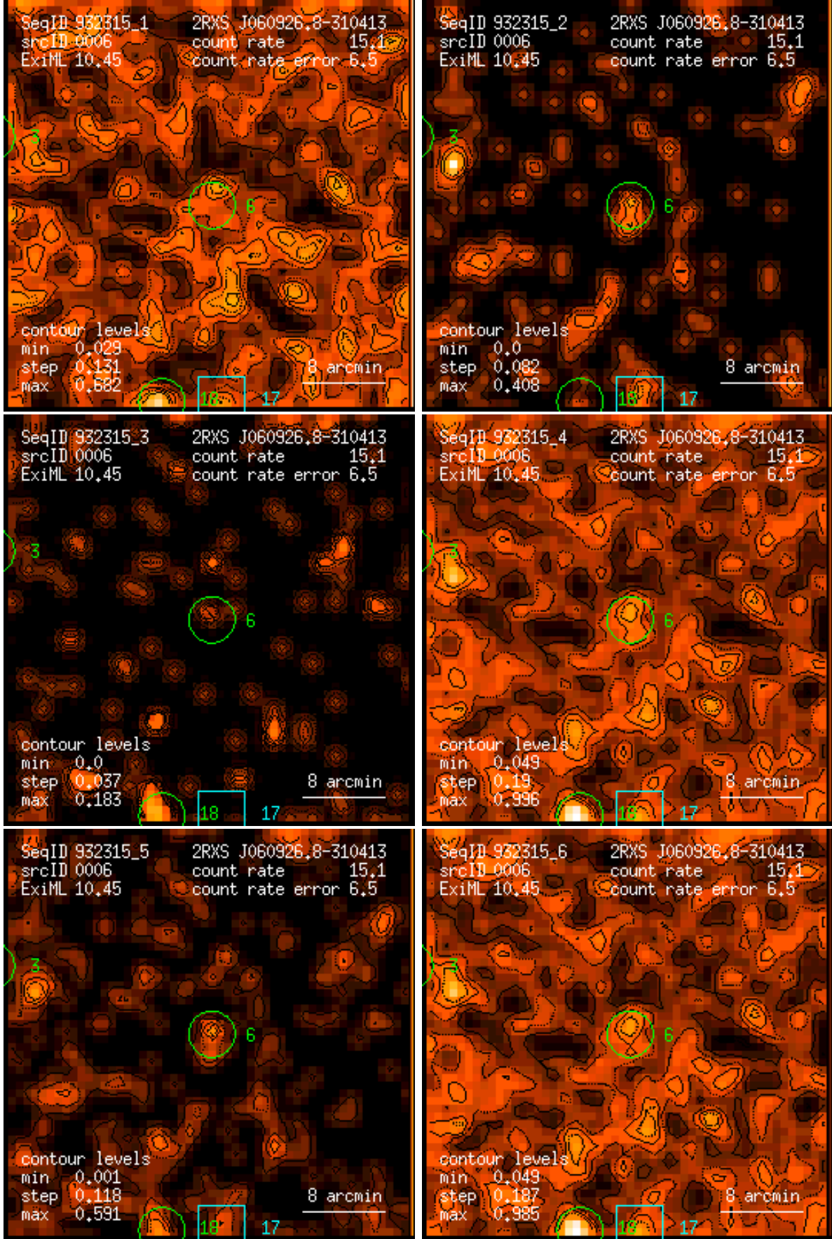
Figure 6: RASS 932315: detection 0006: band rate images, Gaussian filter: (1) PSPC channels 11 – 41, (2) 52 – 90, (3) 91 – 201, (4) 11 – 235, (5) 52 – 201, (6) 11 – 201. Broad band rates in counts/ks. Band rate contour levels in counts/ks/arcmin 2 .
