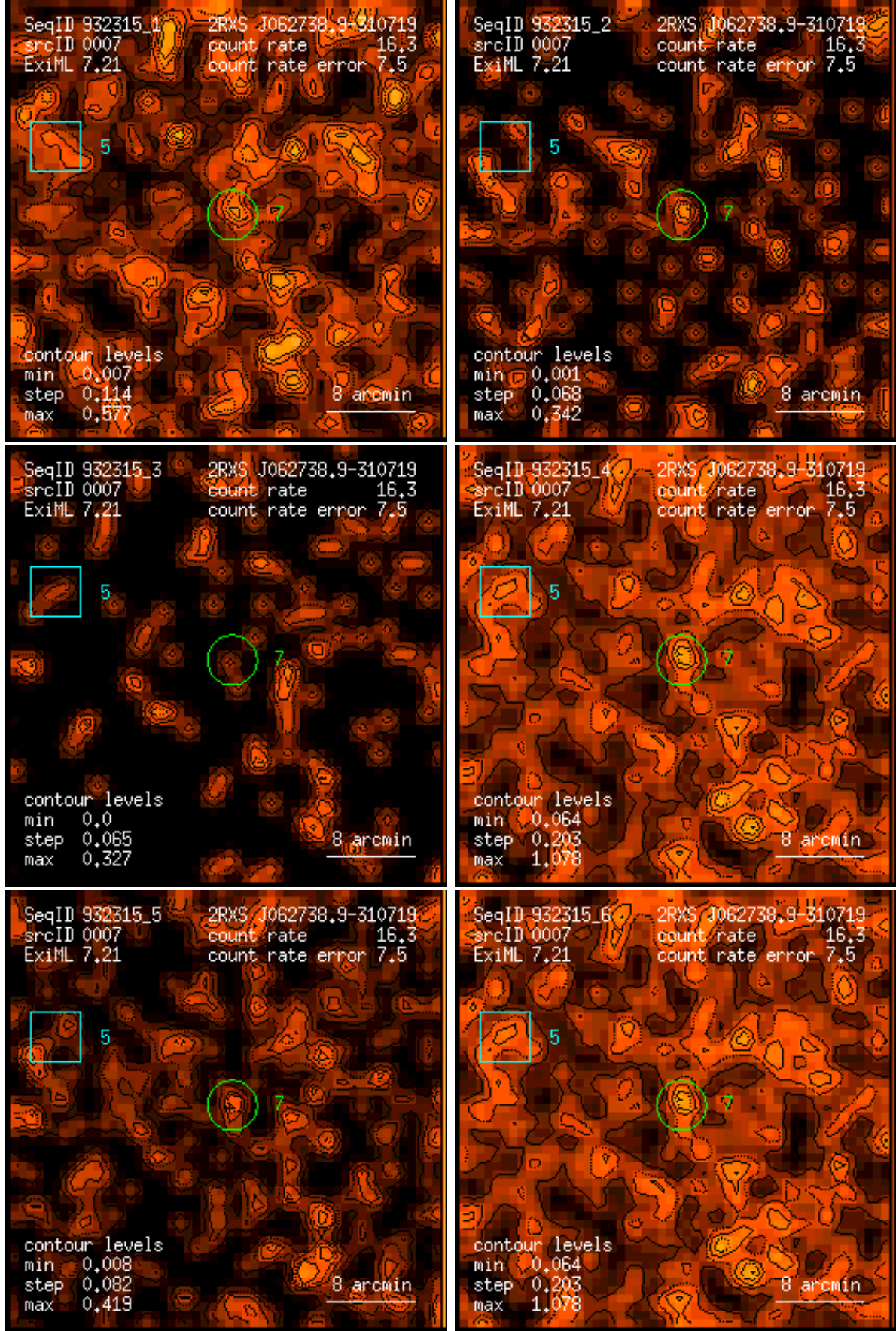
Figure 7: RASS 932315: detection 0007: band rate images, Gaussian filter: (1) PSPC channels 11 – 41, (2) 52 – 90, (3) 91 – 201, (4) 11 – 235, (5) 52 – 201, (6) 11 – 201. Broad band rates in counts/ks. Band rate contour levels in counts/ks/arcmin 2 .
