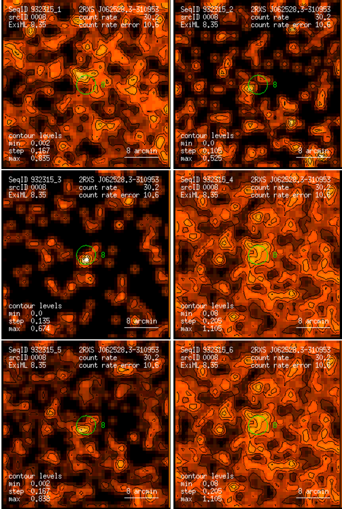
Figure 8: RASS 932315: detection 0008: band rate images, Gaussian filter: (1) PSPC channels 11 – 41, (2) 52 – 90, (3) 91 – 201, (4) 11 – 235, (5) 52 – 201, (6) 11 – 201. Broad band rates in counts/ks. Band rate contour levels in counts/ks/arcmin 2 .
