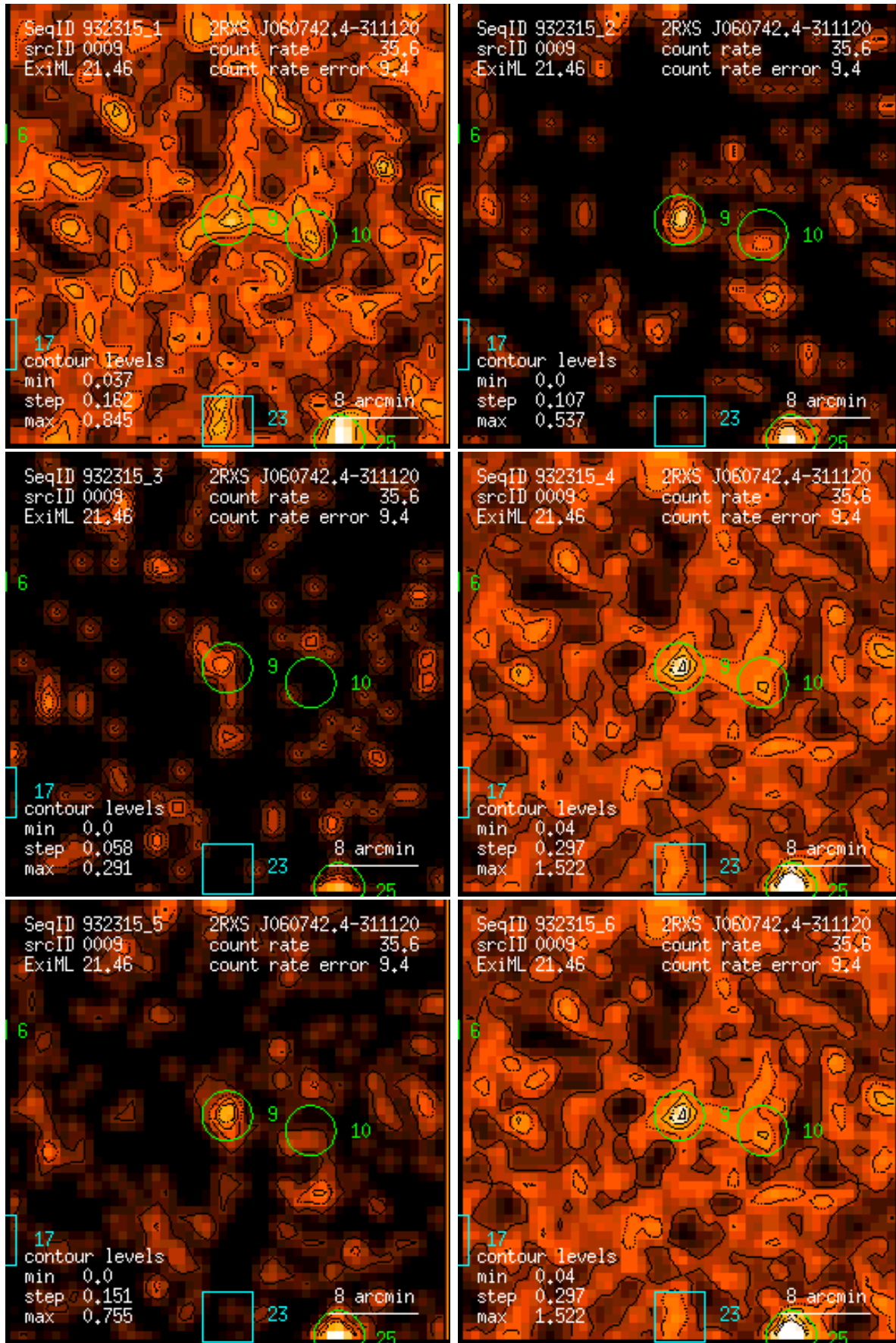
Figure 9: RASS 932315: detection 0009: band rate images, Gaussian filter: (1) PSPC channels 11 – 41, (2) 52 – 90, (3) 91 – 201, (4) 11 – 235, (5) 52 – 201, (6) 11 – 201. Broad band rates in counts/ks. Band rate contour levels in counts/ks/arcmin 2 .
