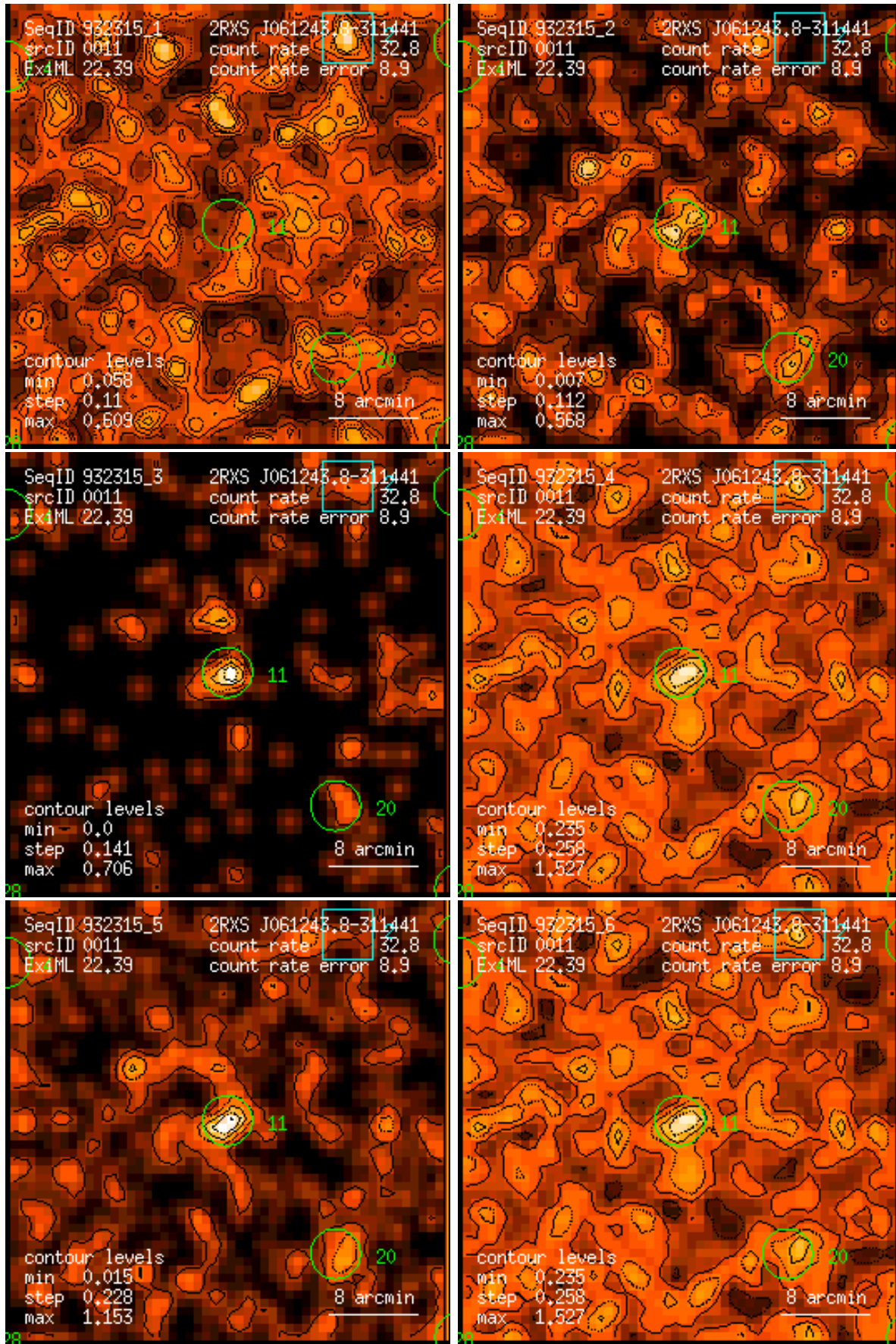
Figure 11: RASS 932315: detection 0011: band rate images, Gaussian filter: (1) PSPC channels 11 – 41, (2) 52 – 90, (3) 91 – 201, (4) 11 – 235, (5) 52 – 201, (6) 11 – 201. Broad band rates in counts/ks. Band rate contour levels in counts/ks/arcmin 2 .
