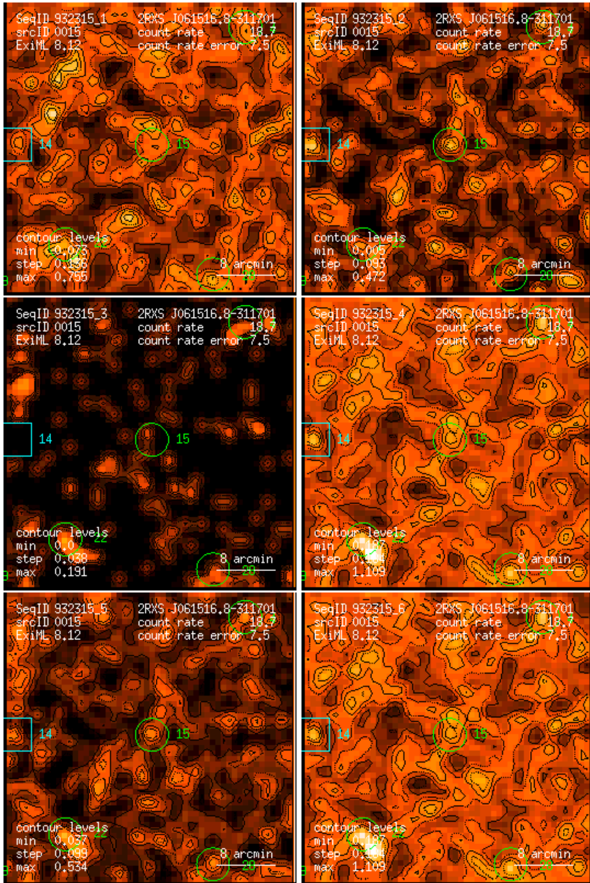
Figure 15: RASS 932315: detection 0015: band rate images, Gaussian filter: (1) PSPC channels 11 – 41, (2) 52 – 90, (3) 91 – 201, (4) 11 – 235, (5) 52 – 201, (6) 11 – 201. Broad band rates in counts/ks. Band rate contour levels in counts/ks/arcmin 2 .
